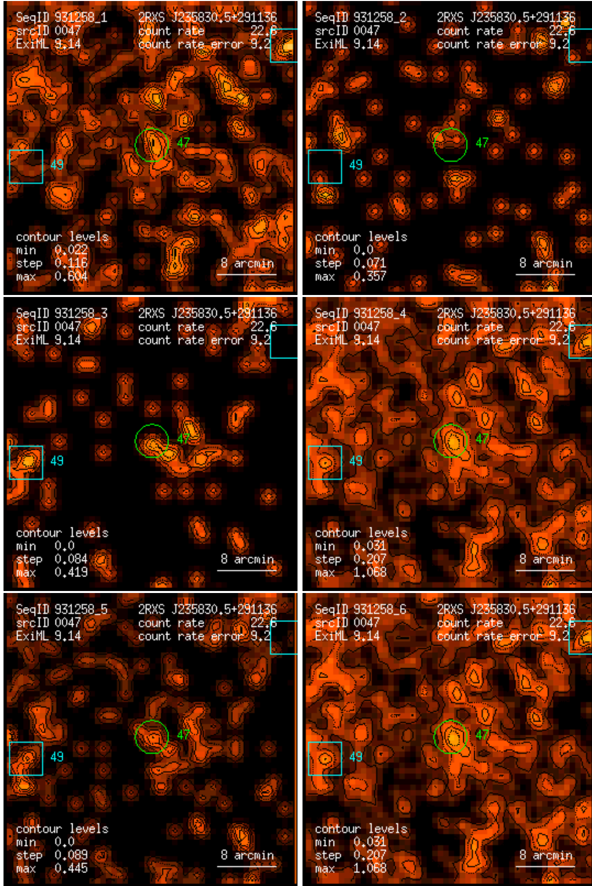
Figure 47: RASS 931258: detection 0047: band rate images, Gaussian filter: (1) PSPC channels 11 – 41, (2) 52 – 90, (3) 91 – 201, (4) 11 – 235, (5) 52 – 201, (6) 11 – 201. Broad band rates in counts/ks. Band rate contour levels in counts/ks/arcmin 2 .
