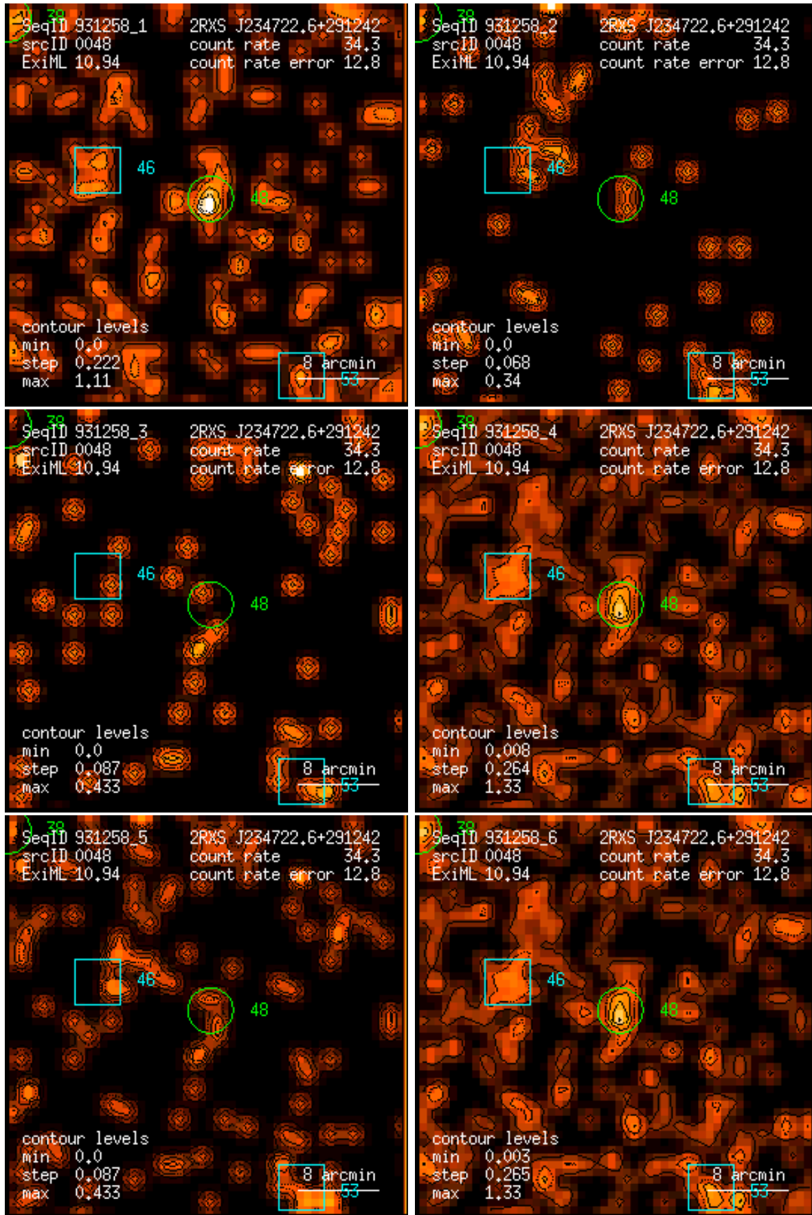
Figure 48: RASS 931258: detection 0048: band rate images, Gaussian filter: (1) PSPC channels 11 – 41, (2) 52 – 90, (3) 91 – 201, (4) 11 – 235, (5) 52 – 201, (6) 11 – 201. Broad band rates in counts/ks. Band rate contour levels in counts/ks/arcmin 2 .
