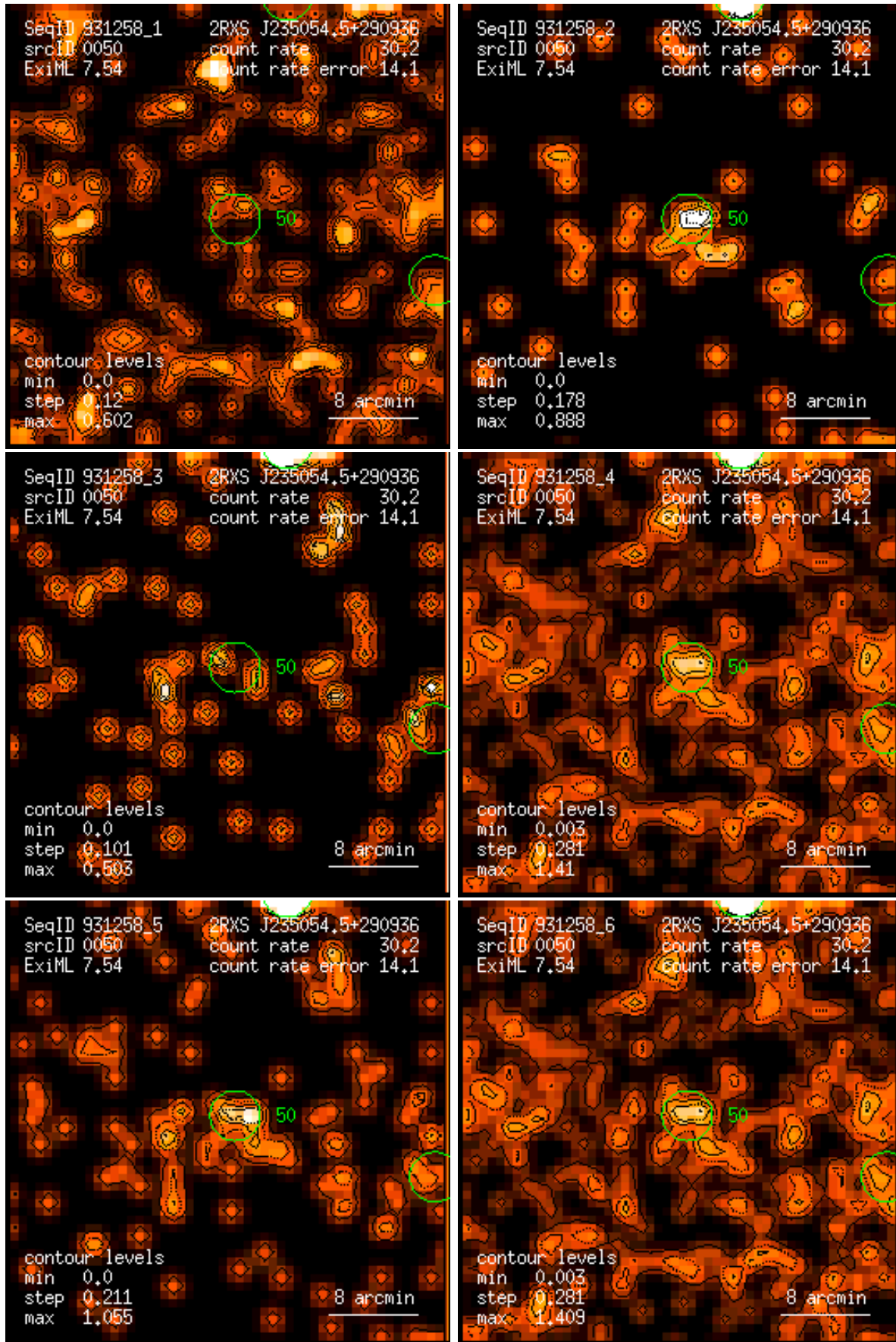
Figure 50: RASS 931258: detection 0050: band rate images, Gaussian filter: (1) PSPC channels 11 – 41, (2) 52 – 90, (3) 91 – 201, (4) 11 – 235, (5) 52 – 201, (6) 11 – 201. Broad band rates in counts/ks. Band rate contour levels in counts/ks/arcmin 2 .
