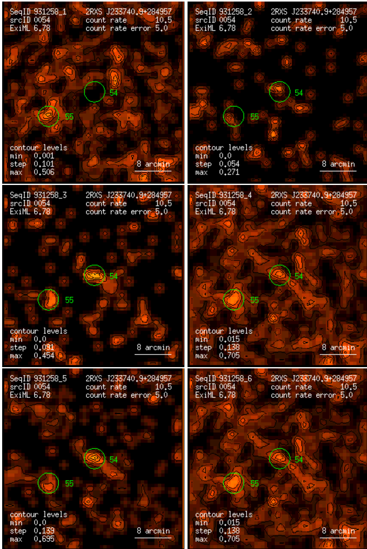
Figure 54: RASS 931258: detection 0054: band rate images, Gaussian filter: (1) PSPC channels 11 – 41, (2) 52 – 90, (3) 91 – 201, (4) 11 – 235, (5) 52 – 201, (6) 11 – 201. Broad band rates in counts/ks. Band rate contour levels in counts/ks/arcmin 2 .
