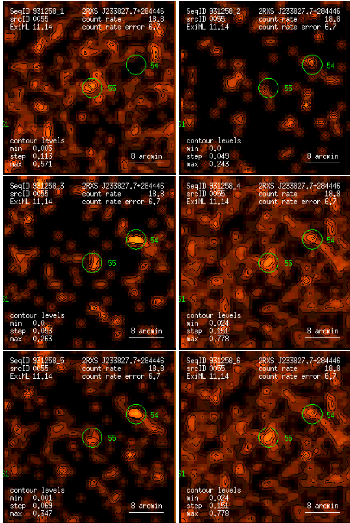
Figure 55: RASS 931258: detection 0055: band rate images, Gaussian filter: (1) PSPC channels 11 – 41, (2) 52 – 90, (3) 91 – 201, (4) 11 – 235, (5) 52 – 201, (6) 11 – 201. Broad band rates in counts/ks. Band rate contour levels in counts/ks/arcmin 2 .
