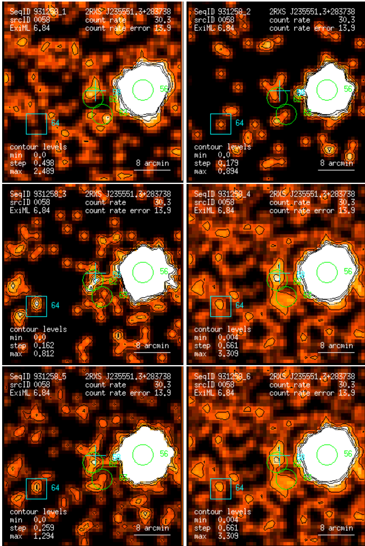
Figure 58: RASS 931258: detection 0058: band rate images, Gaussian filter: (1) PSPC channels 11 – 41, (2) 52 – 90, (3) 91 – 201, (4) 11 – 235, (5) 52 – 201, (6) 11 – 201. Broad band rates in counts/ks. Band rate contour levels in counts/ks/arcmin 2 .
