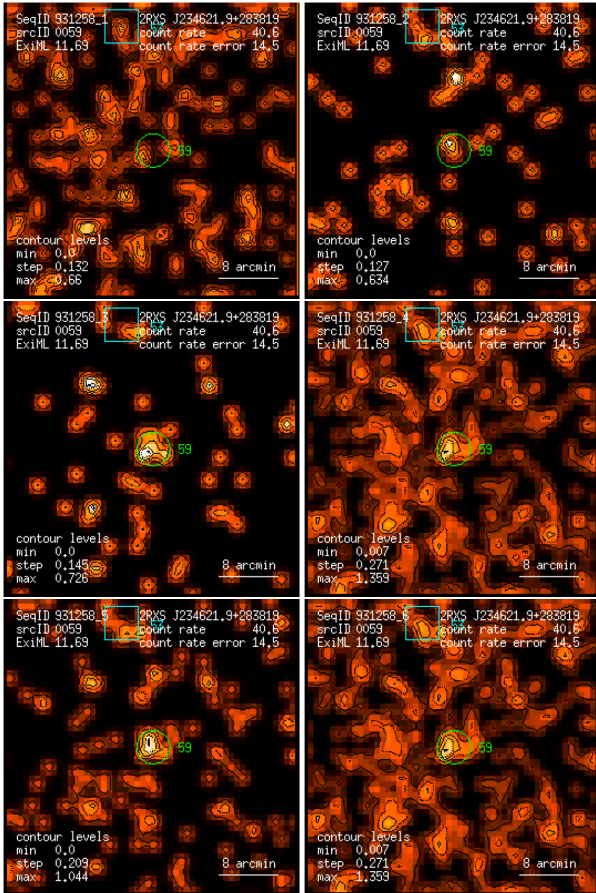
Figure 59: RASS 931258: detection 0059: band rate images, Gaussian filter: (1) PSPC channels 11 – 41, (2) 52 – 90, (3) 91 – 201, (4) 11 – 235, (5) 52 – 201, (6) 11 – 201. Broad band rates in counts/ks. Band rate contour levels in counts/ks/arcmin 2 .
