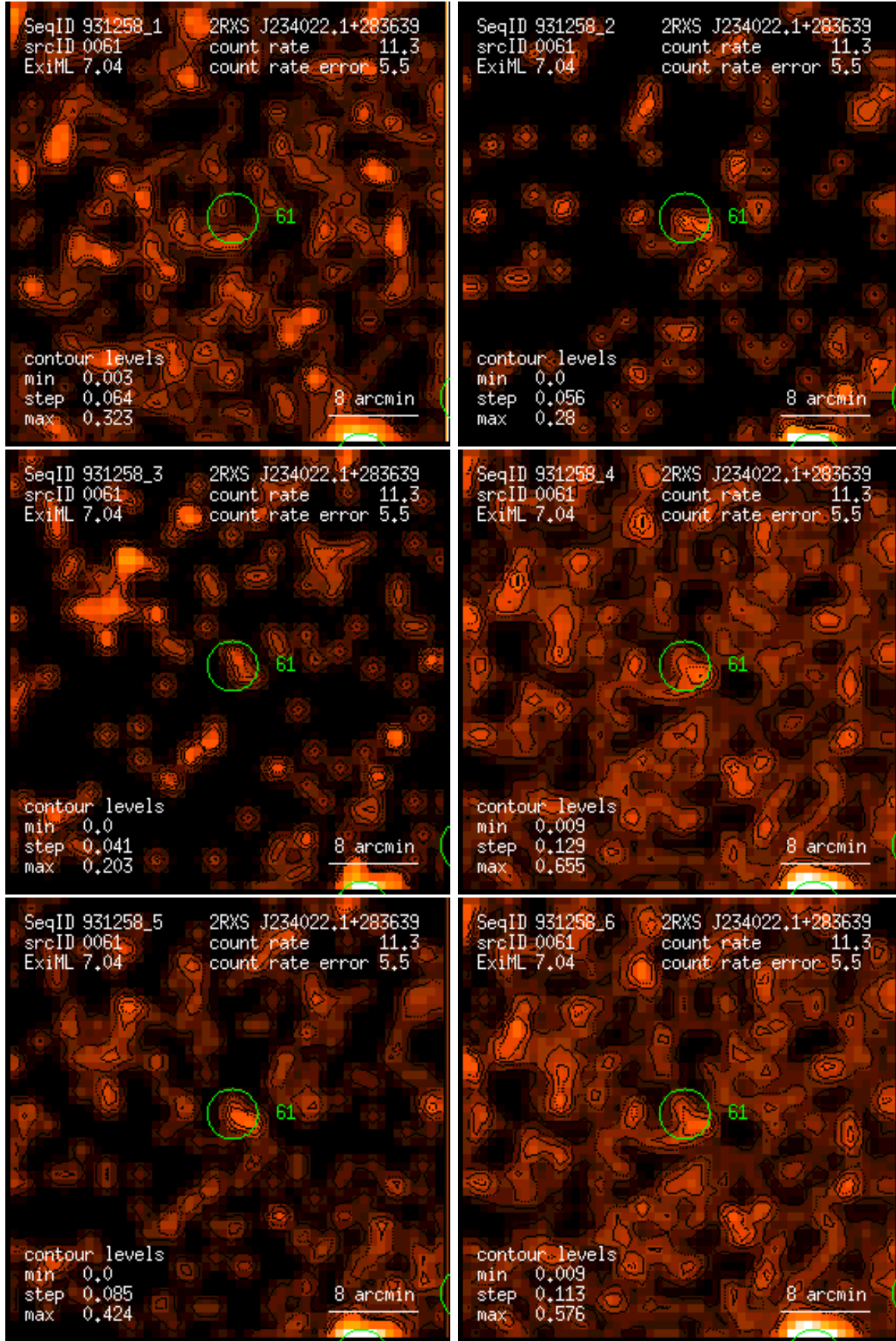
Figure 61: RASS 931258: detection 0061: band rate images, Gaussian filter: (1) PSPC channels 11 – 41, (2) 52 – 90, (3) 91 – 201, (4) 11 – 235, (5) 52 – 201, (6) 11 – 201. Broad band rates in counts/ks. Band rate contour levels in counts/ks/arcmin 2 .
