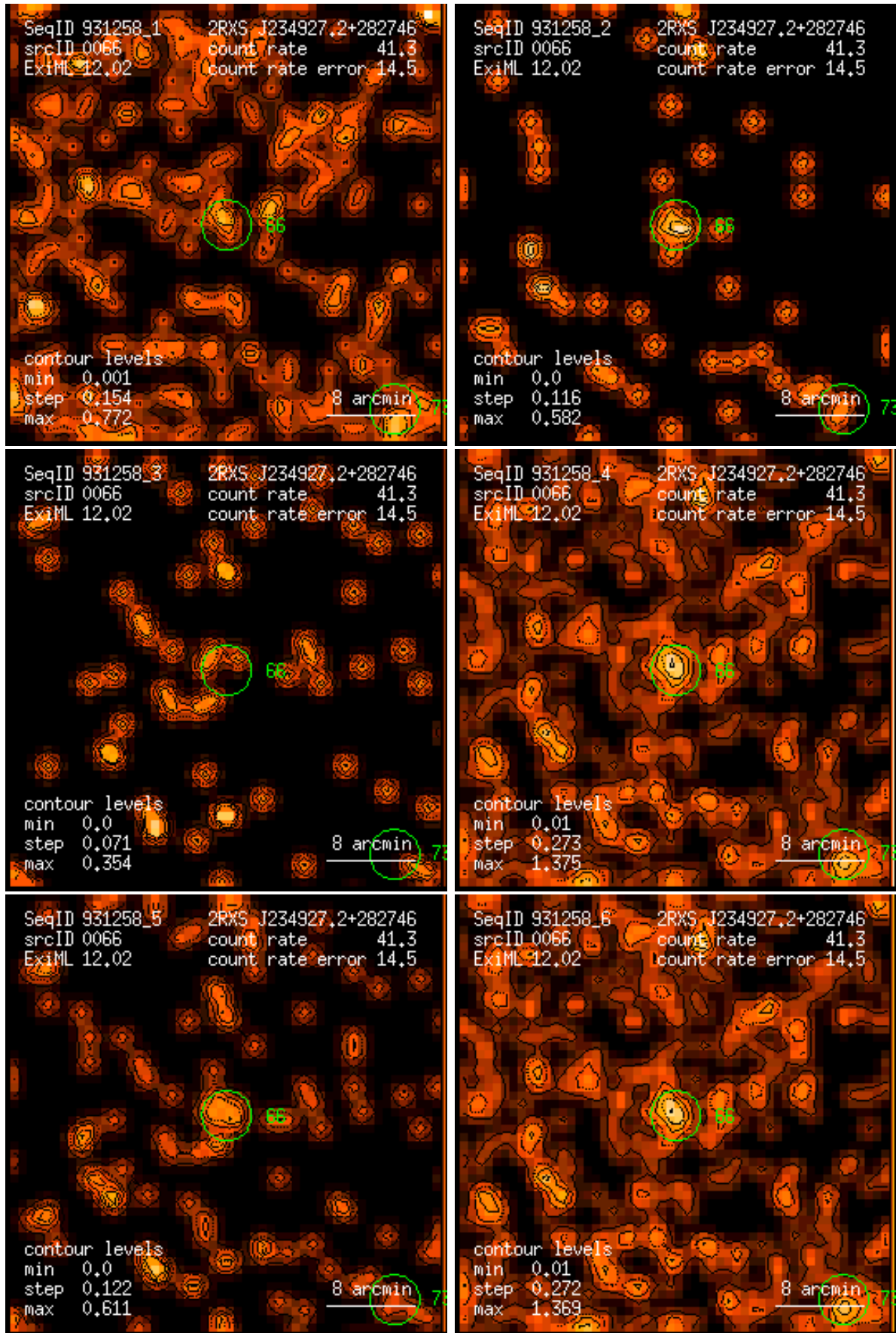
Figure 66: RASS 931258: detection 0066: band rate images, Gaussian filter: (1) PSPC channels 11 – 41, (2) 52 – 90, (3) 91 – 201, (4) 11 – 235, (5) 52 – 201, (6) 11 – 201. Broad band rates in counts/ks. Band rate contour levels in counts/ks/arcmin 2 .
