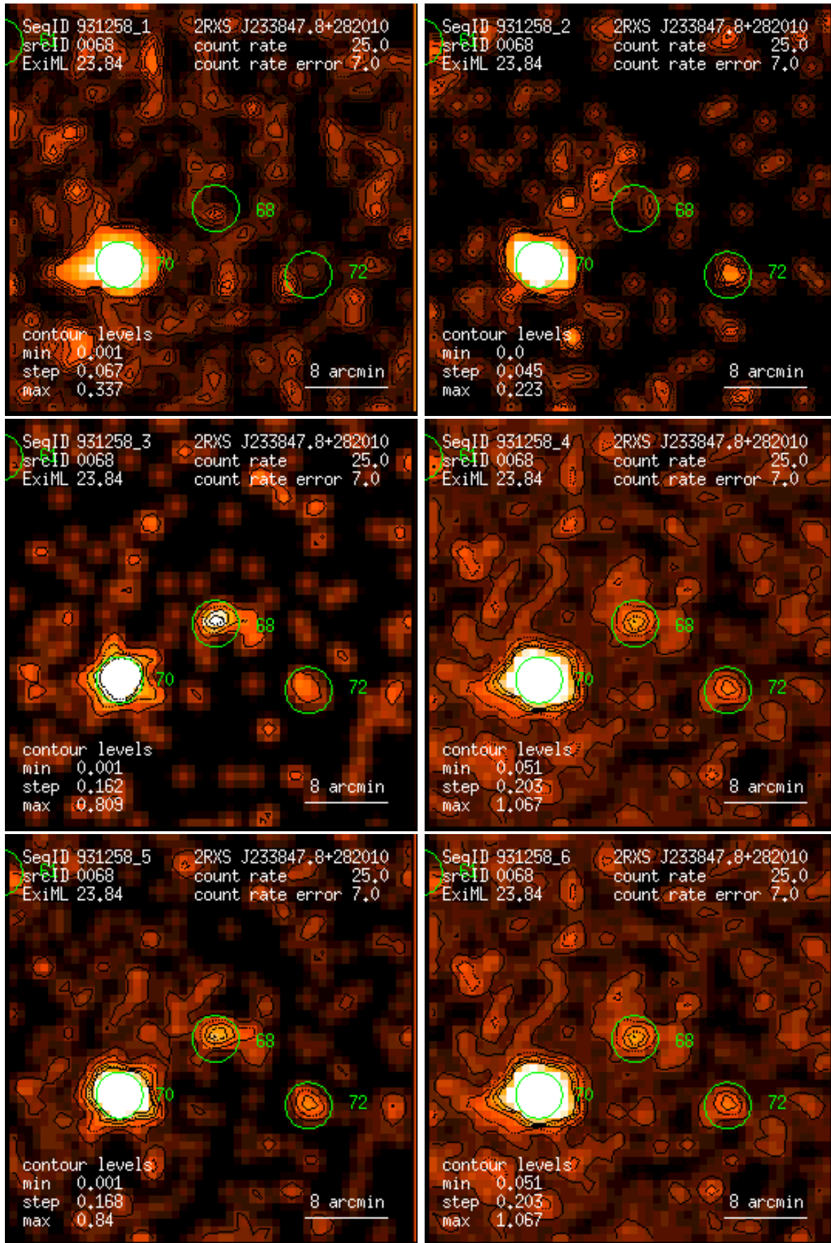
Figure 68: RASS 931258: detection 0068: band rate images, Gaussian filter: (1) PSPC channels 11 – 41, (2) 52 – 90, (3) 91 – 201, (4) 11 – 235, (5) 52 – 201, (6) 11 – 201. Broad band rates in counts/ks. Band rate contour levels in counts/ks/arcmin 2 .
