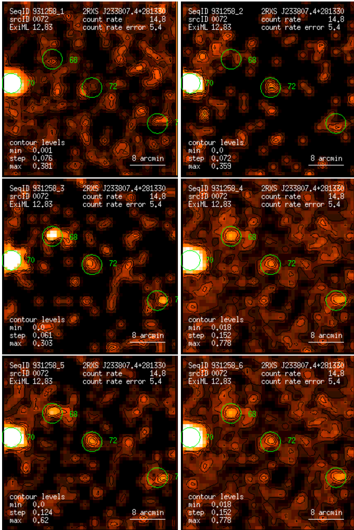
Figure 72: RASS 931258: detection 0072: band rate images, Gaussian filter: (1) PSPC channels 11 – 41, (2) 52 – 90, (3) 91 – 201, (4) 11 – 235, (5) 52 – 201, (6) 11 – 201. Broad band rates in counts/ks. Band rate contour levels in counts/ks/arcmin 2 .
