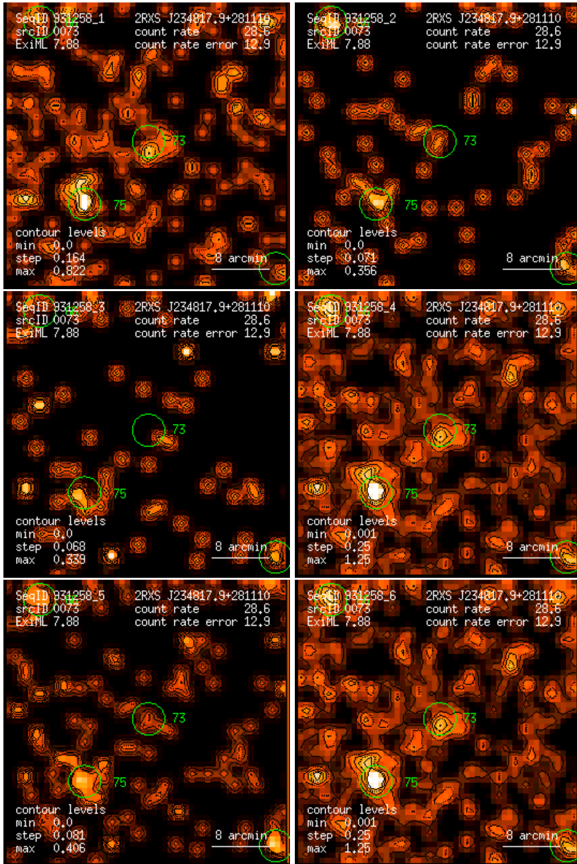
Figure 73: RASS 931258: detection 0073: band rate images, Gaussian filter: (1) PSPC channels 11 – 41, (2) 52 – 90, (3) 91 – 201, (4) 11 – 235, (5) 52 – 201, (6) 11 – 201. Broad band rates in counts/ks. Band rate contour levels in counts/ks/arcmin 2 .
