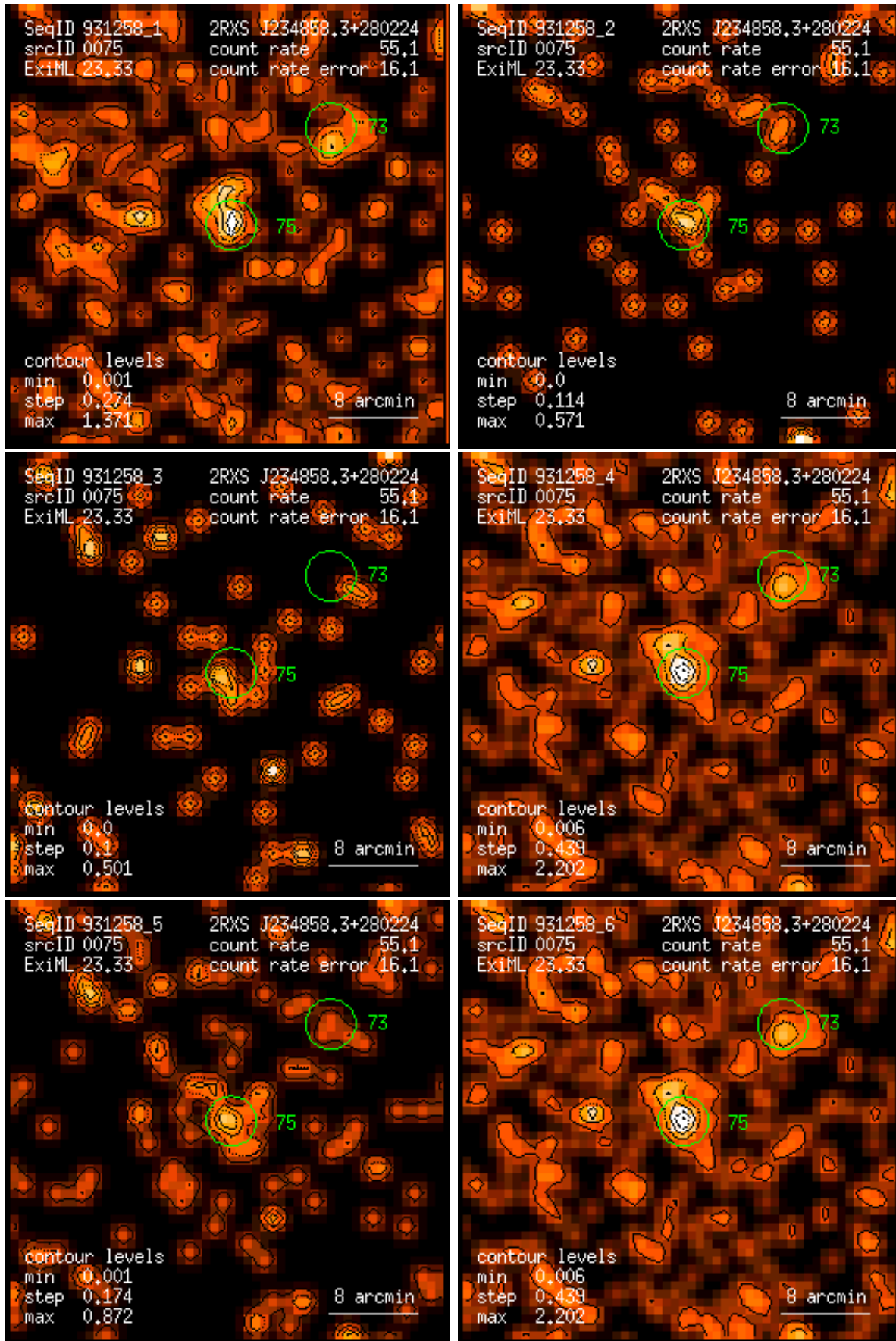
Figure 75: RASS 931258: detection 0075: band rate images, Gaussian filter: (1) PSPC channels 11 – 41, (2) 52 – 90, (3) 91 – 201, (4) 11 – 235, (5) 52 – 201, (6) 11 – 201. Broad band rates in counts/ks. Band rate contour levels in counts/ks/arcmin 2 .
