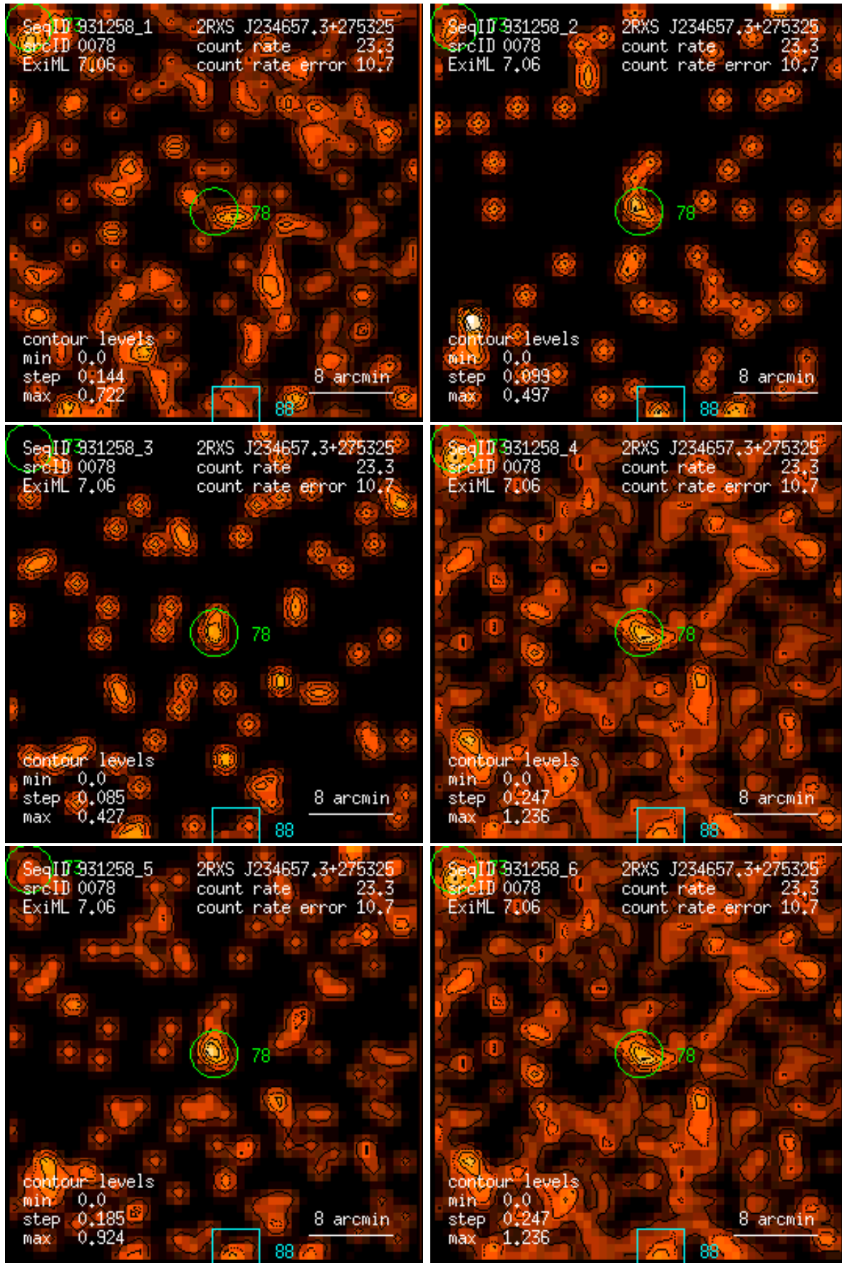
Figure 78: RASS 931258: detection 0078: band rate images, Gaussian filter: (1) PSPC channels 11 – 41, (2) 52 – 90, (3) 91 – 201, (4) 11 – 235, (5) 52 – 201, (6) 11 – 201. Broad band rates in counts/ks. Band rate contour levels in counts/ks/arcmin 2 .
