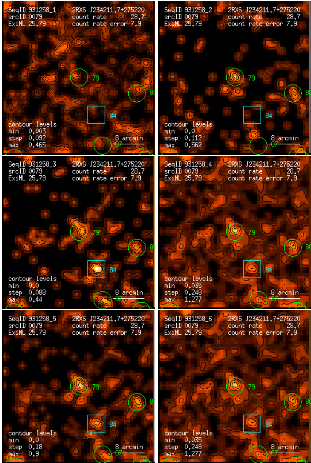
Figure 79: RASS 931258: detection 0079: band rate images, Gaussian filter: (1) PSPC channels 11 – 41, (2) 52 – 90, (3) 91 – 201, (4) 11 – 235, (5) 52 – 201, (6) 11 – 201. Broad band rates in counts/ks. Band rate contour levels in counts/ks/arcmin 2 .
