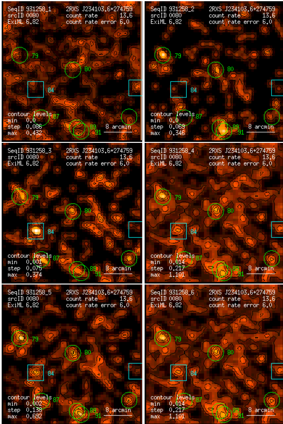
Figure 80: RASS 931258: detection 0080: band rate images, Gaussian filter: (1) PSPC channels 11 – 41, (2) 52 – 90, (3) 91 – 201, (4) 11 – 235, (5) 52 – 201, (6) 11 – 201. Broad band rates in counts/ks. Band rate contour levels in counts/ks/arcmin 2 .
