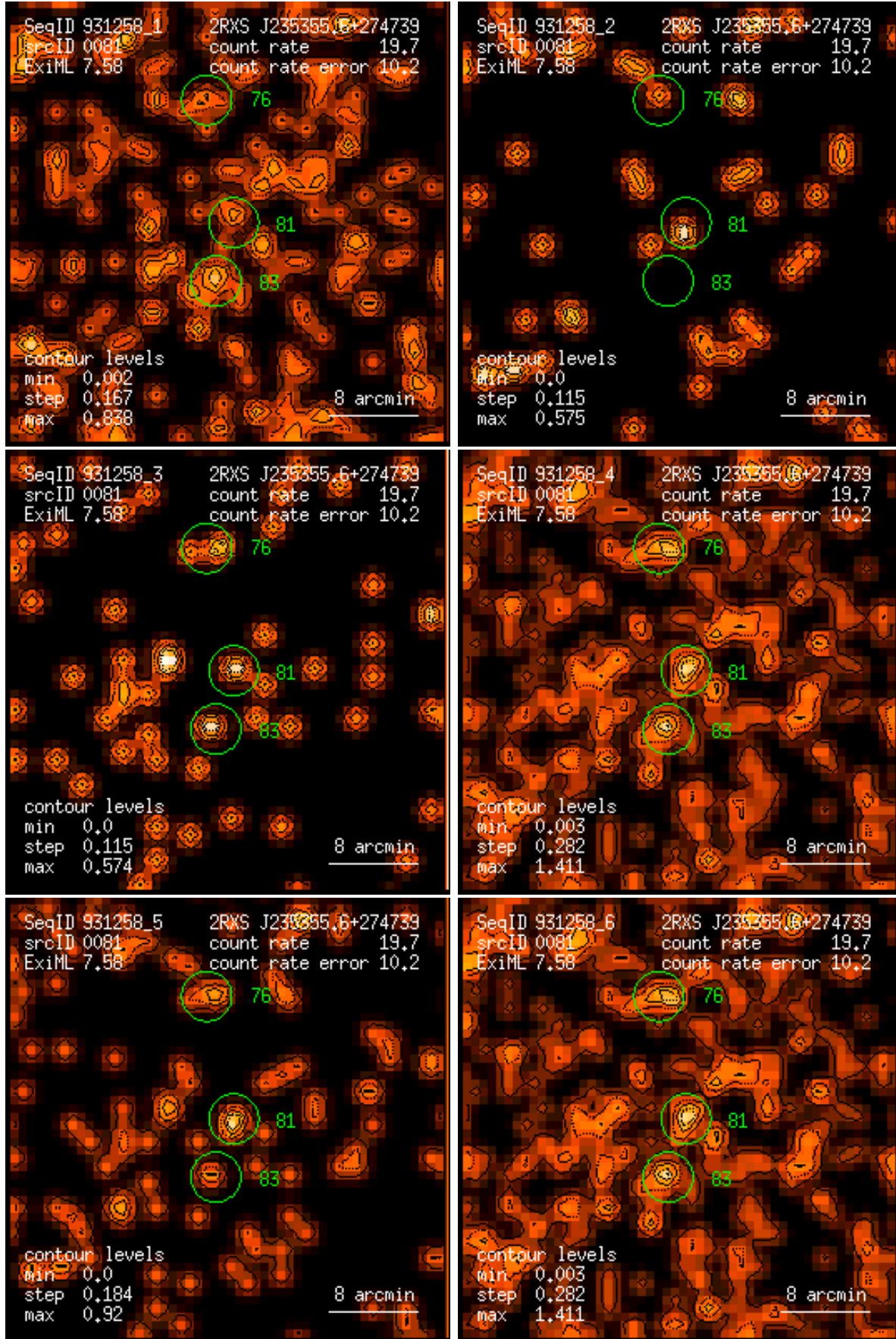
Figure 81: RASS 931258: detection 0081: band rate images, Gaussian filter: (1) PSPC channels 11 – 41, (2) 52 – 90, (3) 91 – 201, (4) 11 – 235, (5) 52 – 201, (6) 11 – 201. Broad band rates in counts/ks. Band rate contour levels in counts/ks/arcmin 2 .
