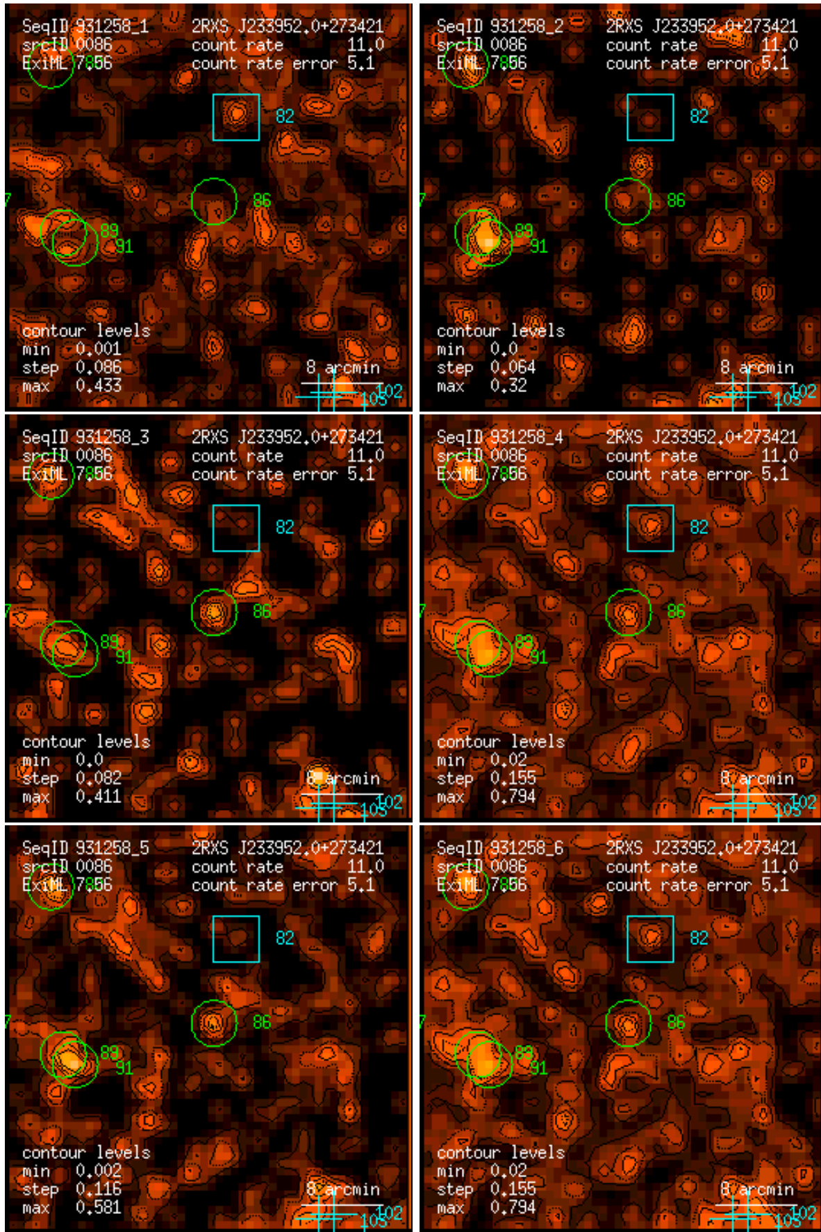
Figure 86: RASS 931258: detection 0086: band rate images, Gaussian filter: (1) PSPC channels 11 – 41, (2) 52 – 90, (3) 91 – 201, (4) 11 – 235, (5) 52 – 201, (6) 11 – 201. Broad band rates in counts/ks. Band rate contour levels in counts/ks/arcmin 2 .
