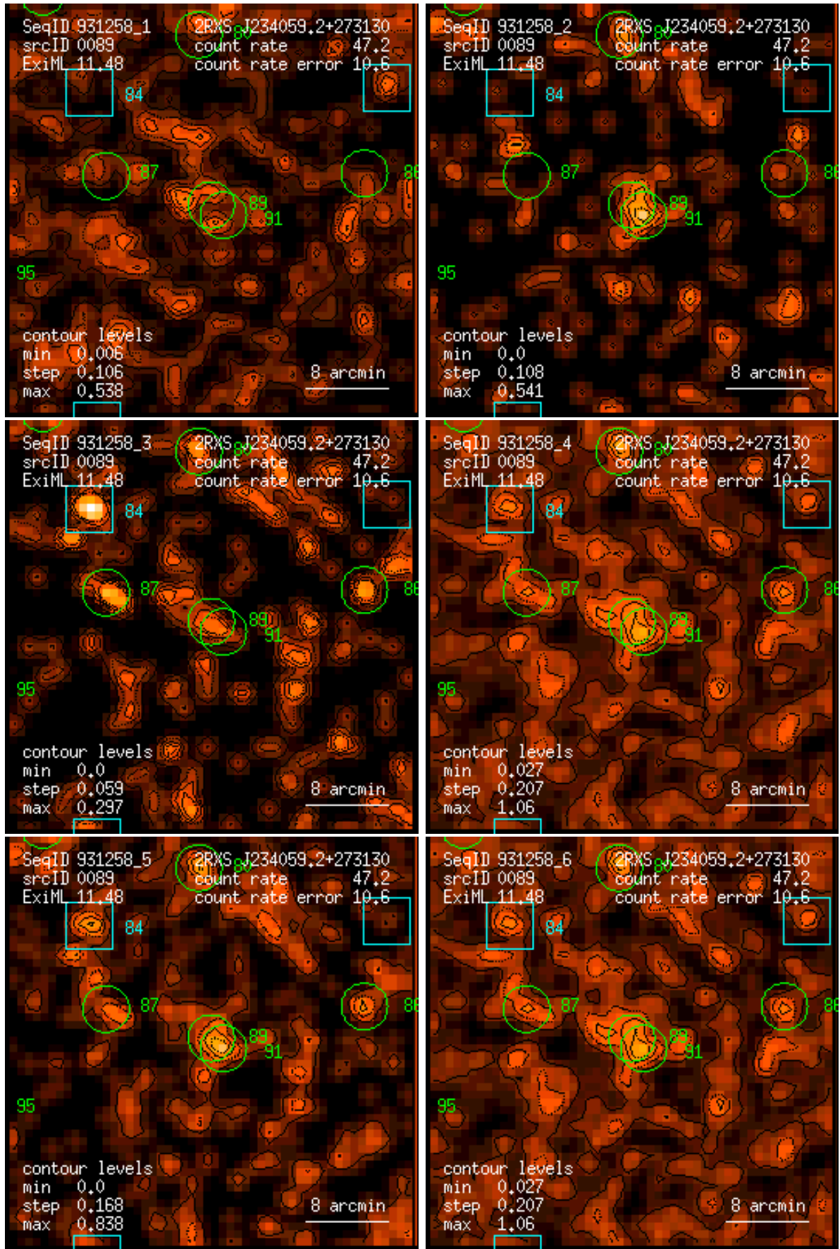
Figure 89: RASS 931258: detection 0089: band rate images, Gaussian filter: (1) PSPC channels 11 – 41, (2) 52 – 90, (3) 91 – 201, (4) 11 – 235, (5) 52 – 201, (6) 11 – 201. Broad band rates in counts/ks. Band rate contour levels in counts/ks/arcmin 2 .
