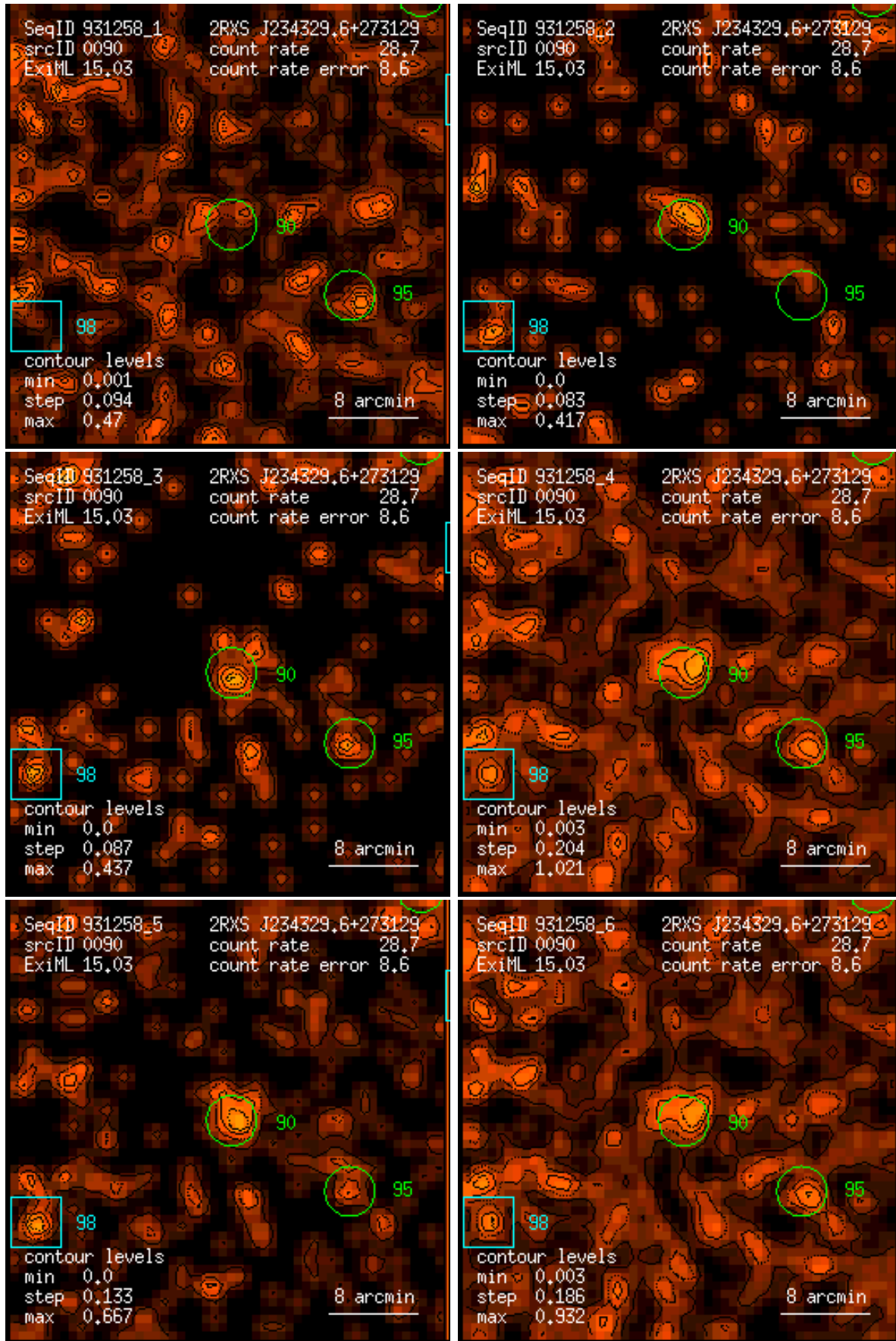
Figure 90: RASS 931258: detection 0090: band rate images, Gaussian filter: (1) PSPC channels 11 – 41, (2) 52 – 90, (3) 91 – 201, (4) 11 – 235, (5) 52 – 201, (6) 11 – 201. Broad band rates in counts/ks. Band rate contour levels in counts/ks/arcmin 2 .
