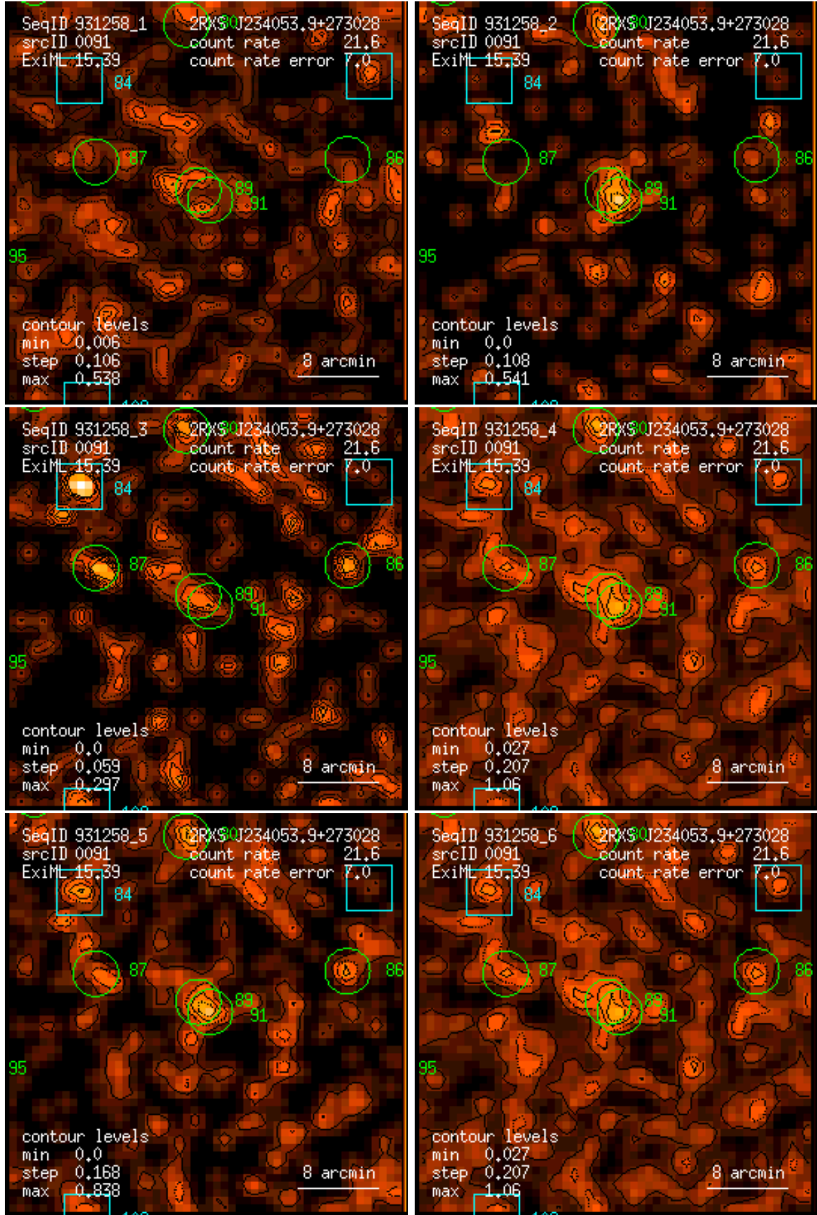
Figure 91: RASS 931258: detection 0091: band rate images, Gaussian filter: (1) PSPC channels 11 – 41, (2) 52 – 90, (3) 91 – 201, (4) 11 – 235, (5) 52 – 201, (6) 11 – 201. Broad band rates in counts/ks. Band rate contour levels in counts/ks/arcmin 2 .
