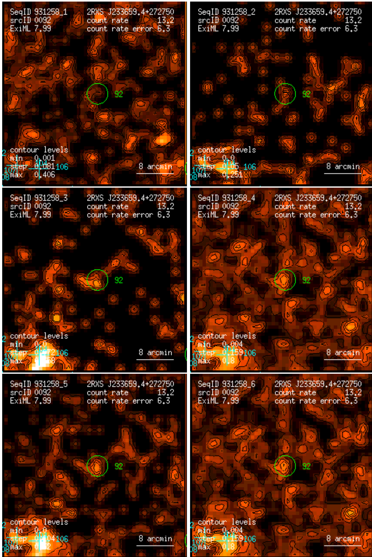
Figure 92: RASS 931258: detection 0092: band rate images, Gaussian filter: (1) PSPC channels 11 – 41, (2) 52 – 90, (3) 91 – 201, (4) 11 – 235, (5) 52 – 201, (6) 11 – 201. Broad band rates in counts/ks. Band rate contour levels in counts/ks/arcmin 2 .
