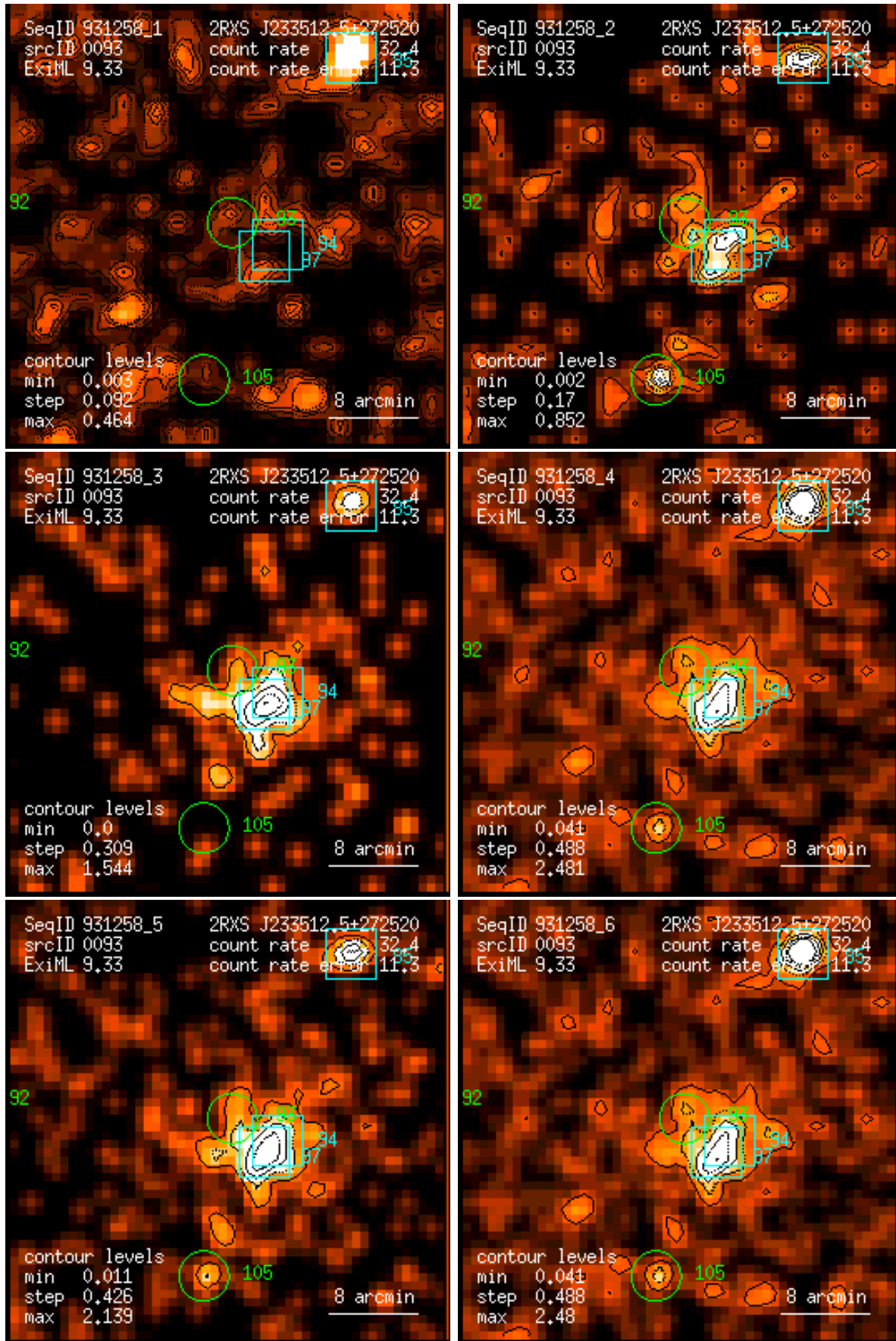
Figure 93: RASS 931258: detection 0093: band rate images, Gaussian filter: (1) PSPC channels 11 – 41, (2) 52 – 90, (3) 91 – 201, (4) 11 – 235, (5) 52 – 201, (6) 11 – 201. Broad band rates in counts/ks. Band rate contour levels in counts/ks/arcmin 2 .
