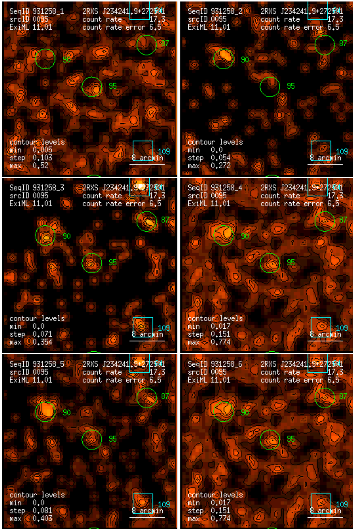
Figure 95: RASS 931258: detection 0095: band rate images, Gaussian filter: (1) PSPC channels 11 – 41, (2) 52 – 90, (3) 91 – 201, (4) 11 – 235, (5) 52 – 201, (6) 11 – 201. Broad band rates in counts/ks. Band rate contour levels in counts/ks/arcmin 2 .
