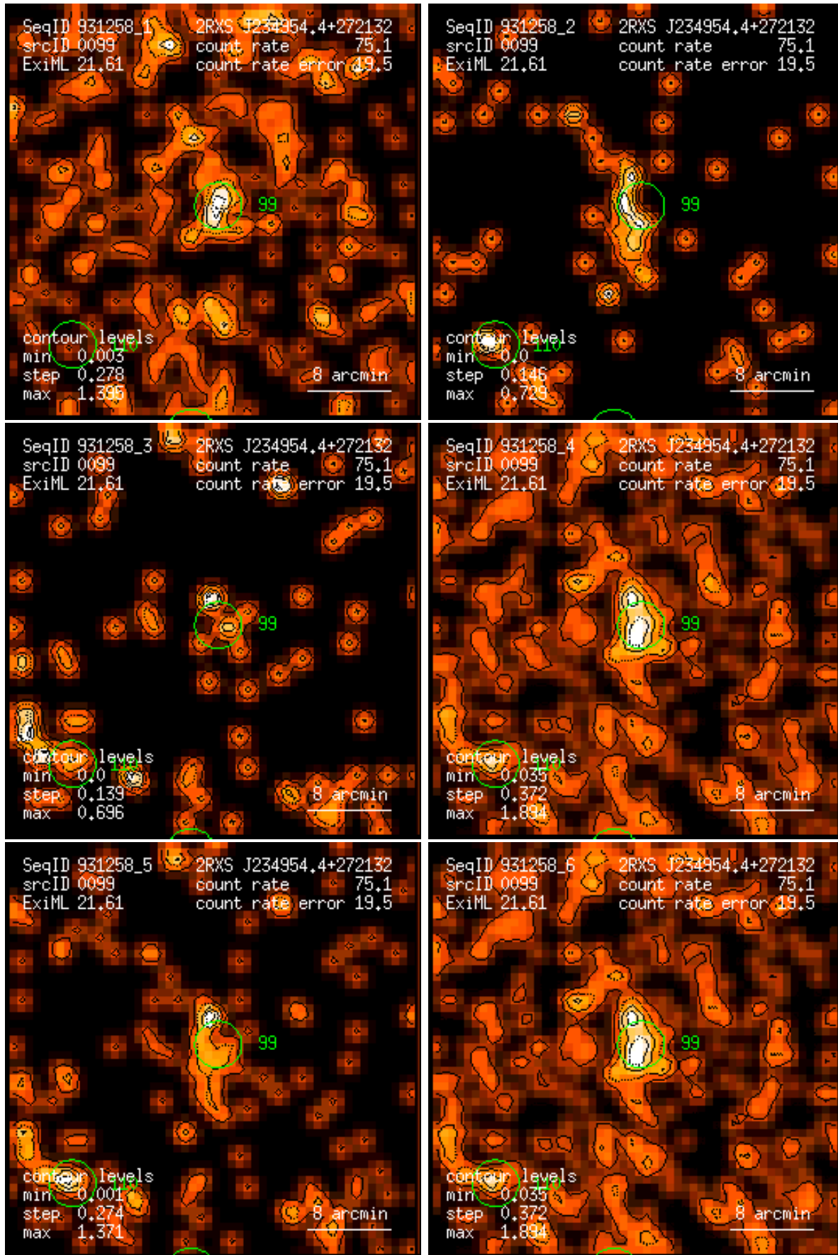
Figure 99: RASS 931258: detection 0099: band rate images, Gaussian filter: (1) PSPC channels 11 – 41, (2) 52 – 90, (3) 91 – 201, (4) 11 – 235, (5) 52 – 201, (6) 11 – 201. Broad band rates in counts/ks. Band rate contour levels in counts/ks/arcmin 2 .
