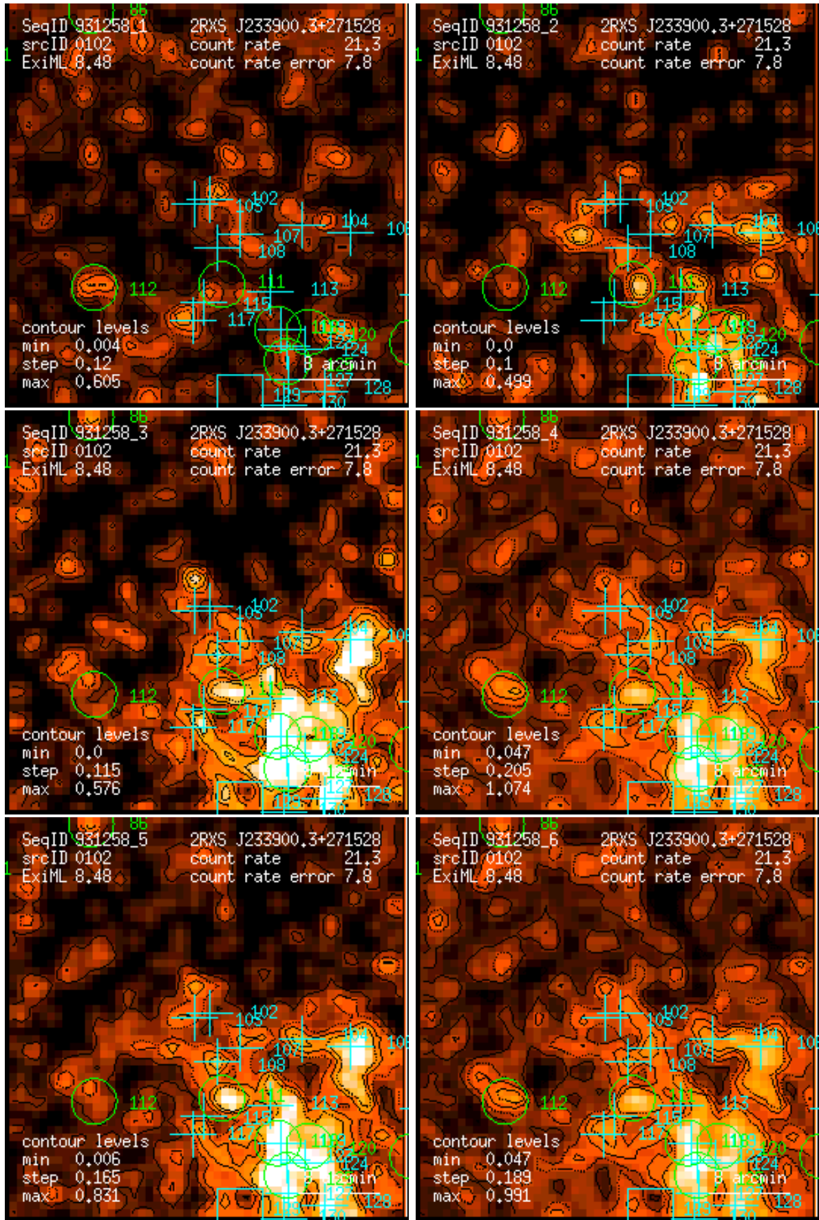
Figure 102: RASS 931258: detection 0102: band rate images, Gaussian filter: (1) PSPC channels 11 – 41, (2) 52 – 90, (3) 91 – 201, (4) 11 – 235, (5) 52 – 201, (6) 11 – 201. Broad band rates in counts/ks. Band rate contour levels in counts/ks/arcmin 2 .
