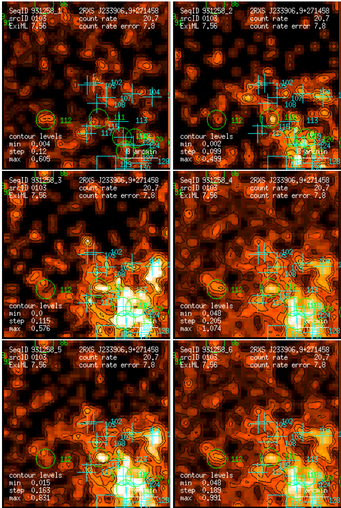
Figure 103: RASS 931258: detection 0103: band rate images, Gaussian filter: (1) PSPC channels 11 – 41, (2) 52 – 90, (3) 91 – 201, (4) 11 – 235, (5) 52 – 201, (6) 11 – 201. Broad band rates in counts/ks. Band rate contour levels in counts/ks/arcmin 2 .
