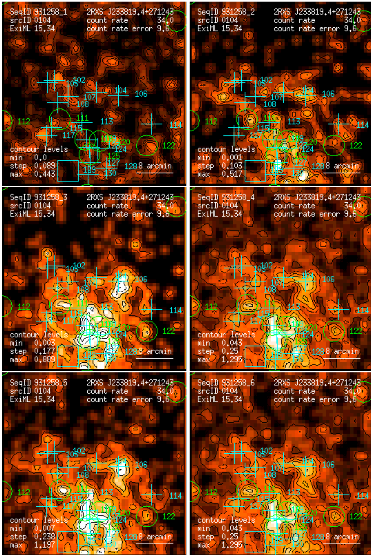
Figure 104: RASS 931258: detection 0104: band rate images, Gaussian filter: (1) PSPC channels 11 – 41, (2) 52 – 90, (3) 91 – 201, (4) 11 – 235, (5) 52 – 201, (6) 11 – 201. Broad band rates in counts/ks. Band rate contour levels in counts/ks/arcmin 2 .
