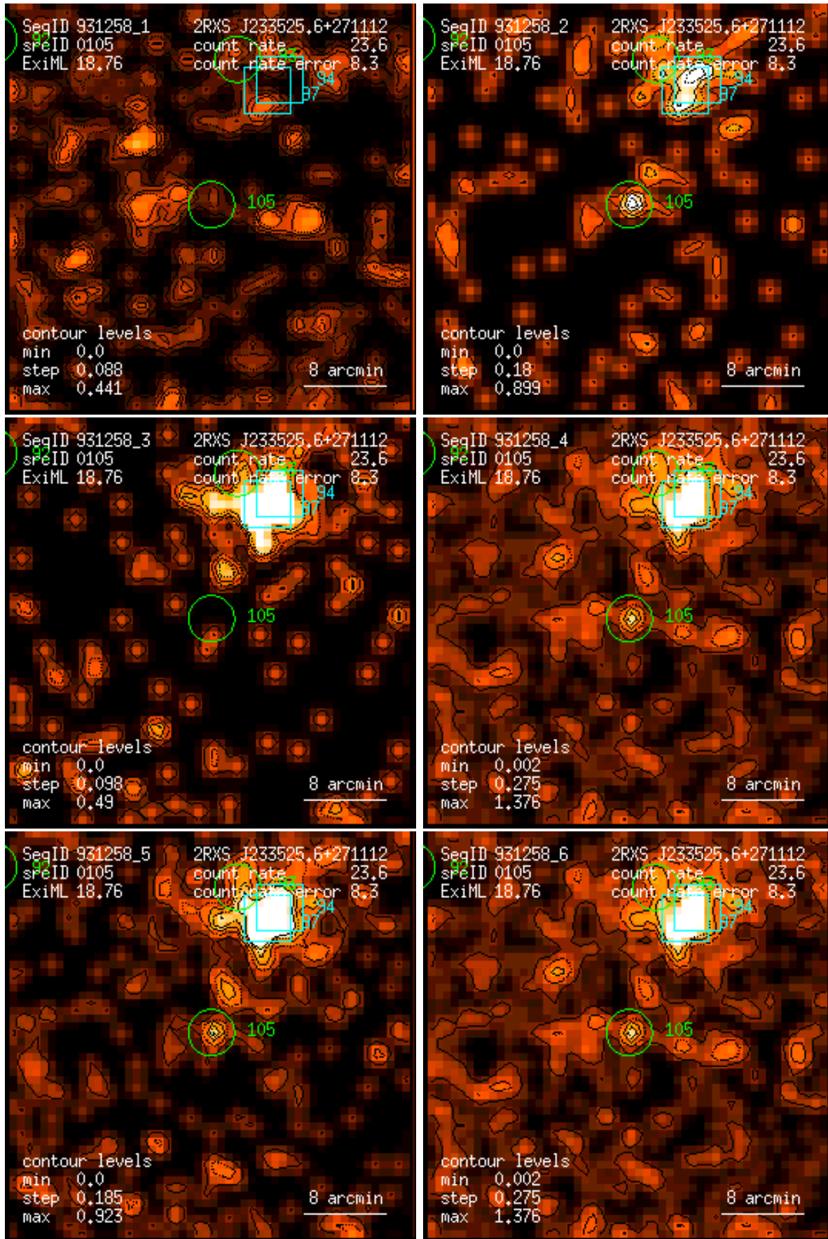
Figure 105: RASS 931258: detection 0105: band rate images, Gaussian filter: (1) PSPC channels 11 – 41, (2) 52 – 90, (3) 91 – 201, (4) 11 – 235, (5) 52 – 201, (6) 11 – 201. Broad band rates in counts/ks. Band rate contour levels in counts/ks/arcmin 2 .
