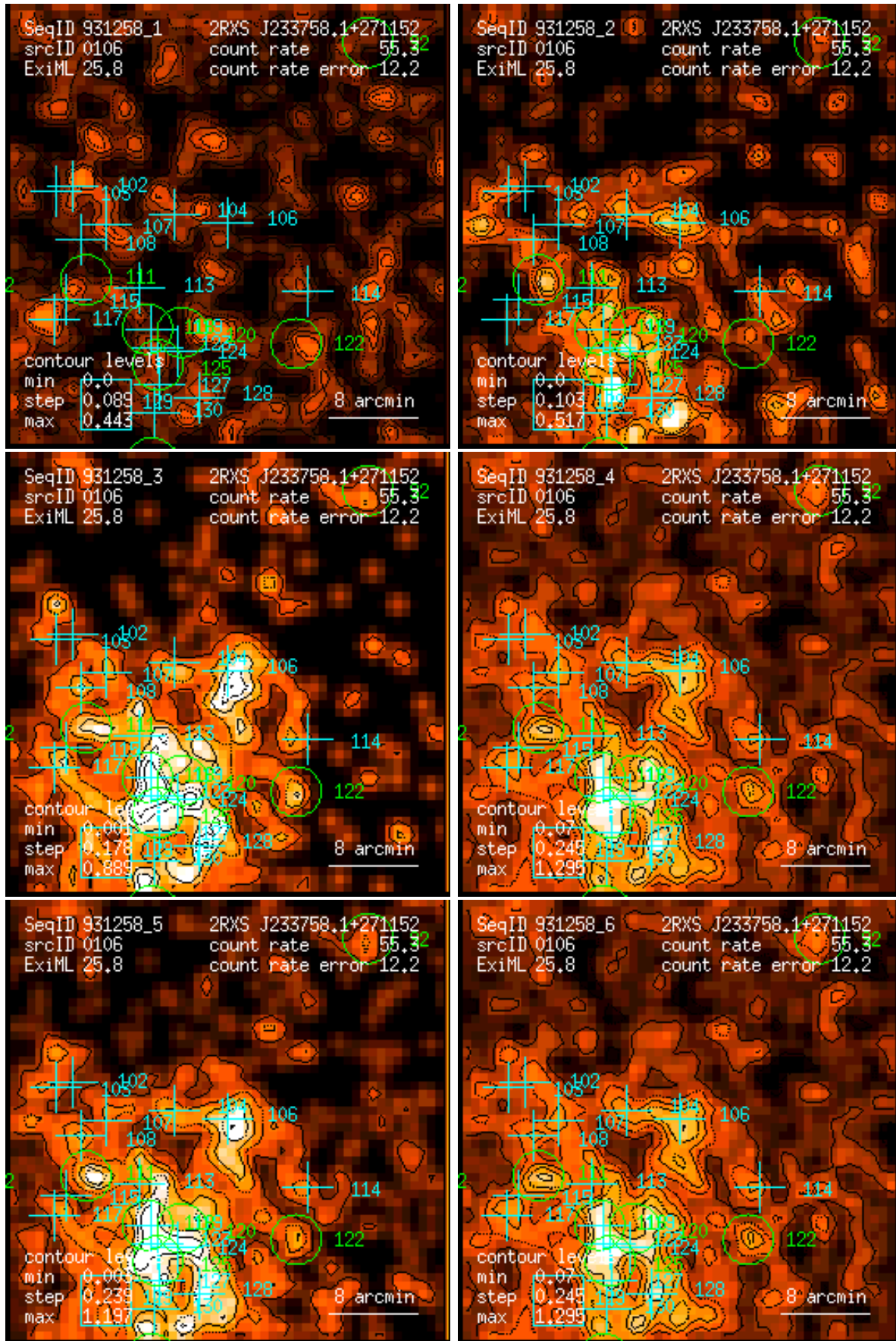
Figure 106: RASS 931258: detection 0106: band rate images, Gaussian filter: (1) PSPC channels 11 – 41, (2) 52 – 90, (3) 91 – 201, (4) 11 – 235, (5) 52 – 201, (6) 11 – 201. Broad band rates in counts/ks. Band rate contour levels in counts/ks/arcmin 2 .
