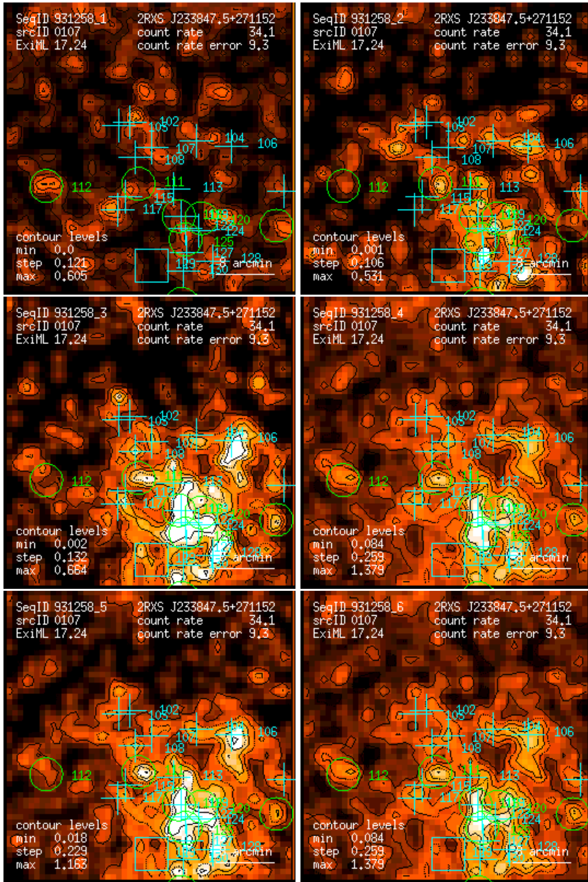
Figure 107: RASS 931258: detection 0107: band rate images, Gaussian filter: (1) PSPC channels 11 – 41, (2) 52 – 90, (3) 91 – 201, (4) 11 – 235, (5) 52 – 201, (6) 11 – 201. Broad band rates in counts/ks. Band rate contour levels in counts/ks/arcmin 2 .
