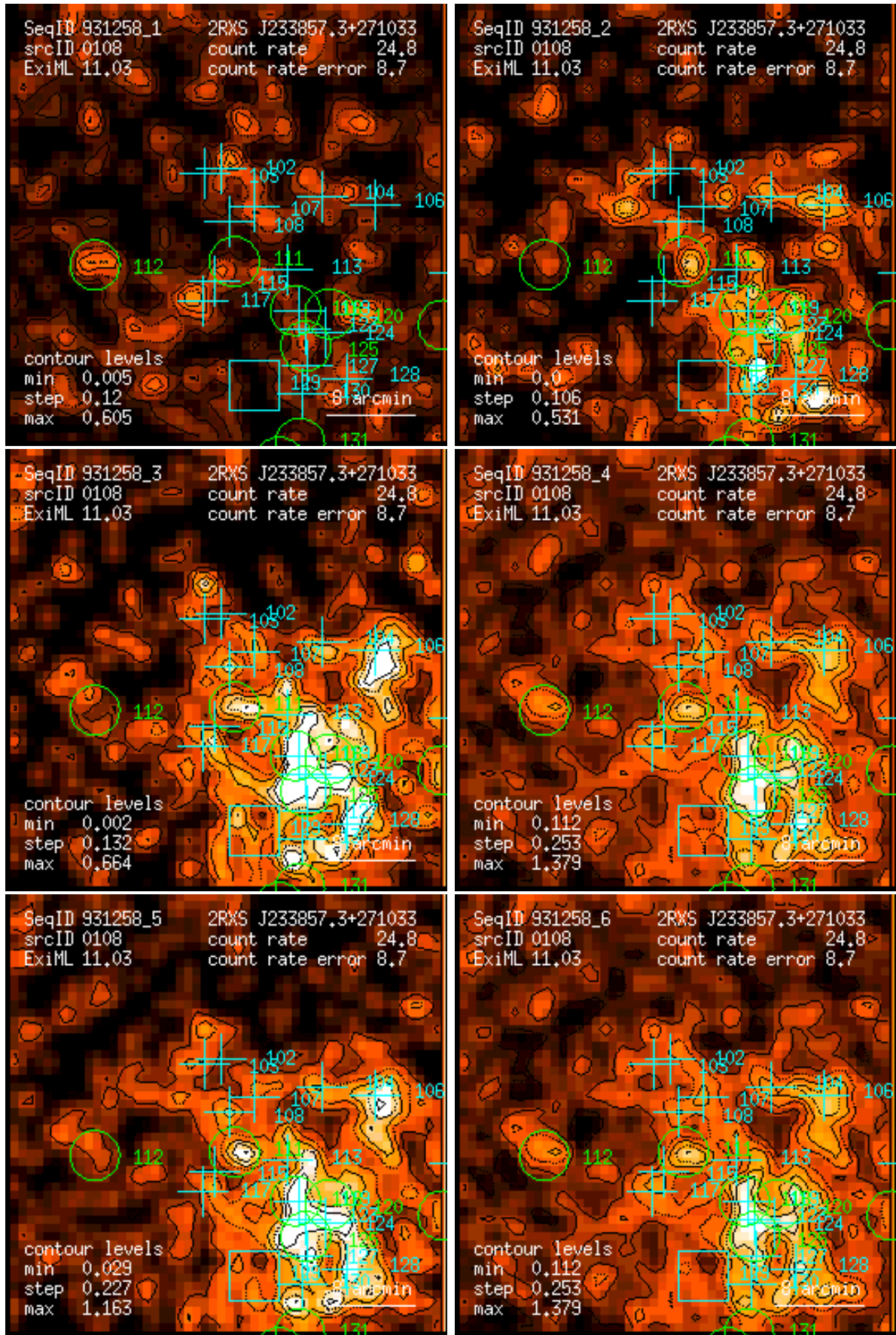
Figure 108: RASS 931258: detection 0108: band rate images, Gaussian filter: (1) PSPC channels 11 – 41, (2) 52 – 90, (3) 91 – 201, (4) 11 – 235, (5) 52 – 201, (6) 11 – 201. Broad band rates in counts/ks. Band rate contour levels in counts/ks/arcmin 2 .
