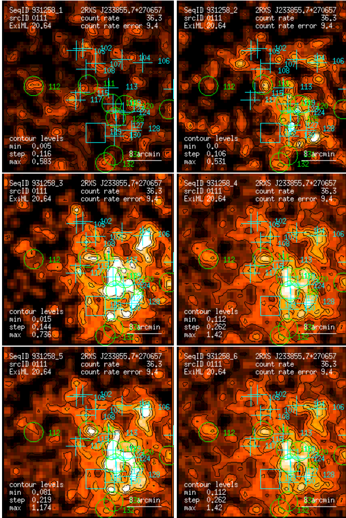
Figure 111: RASS 931258: detection 0111: band rate images, Gaussian filter: (1) PSPC channels 11 – 41, (2) 52 – 90, (3) 91 – 201, (4) 11 – 235, (5) 52 – 201, (6) 11 – 201. Broad band rates in counts/ks. Band rate contour levels in counts/ks/arcmin 2 .
