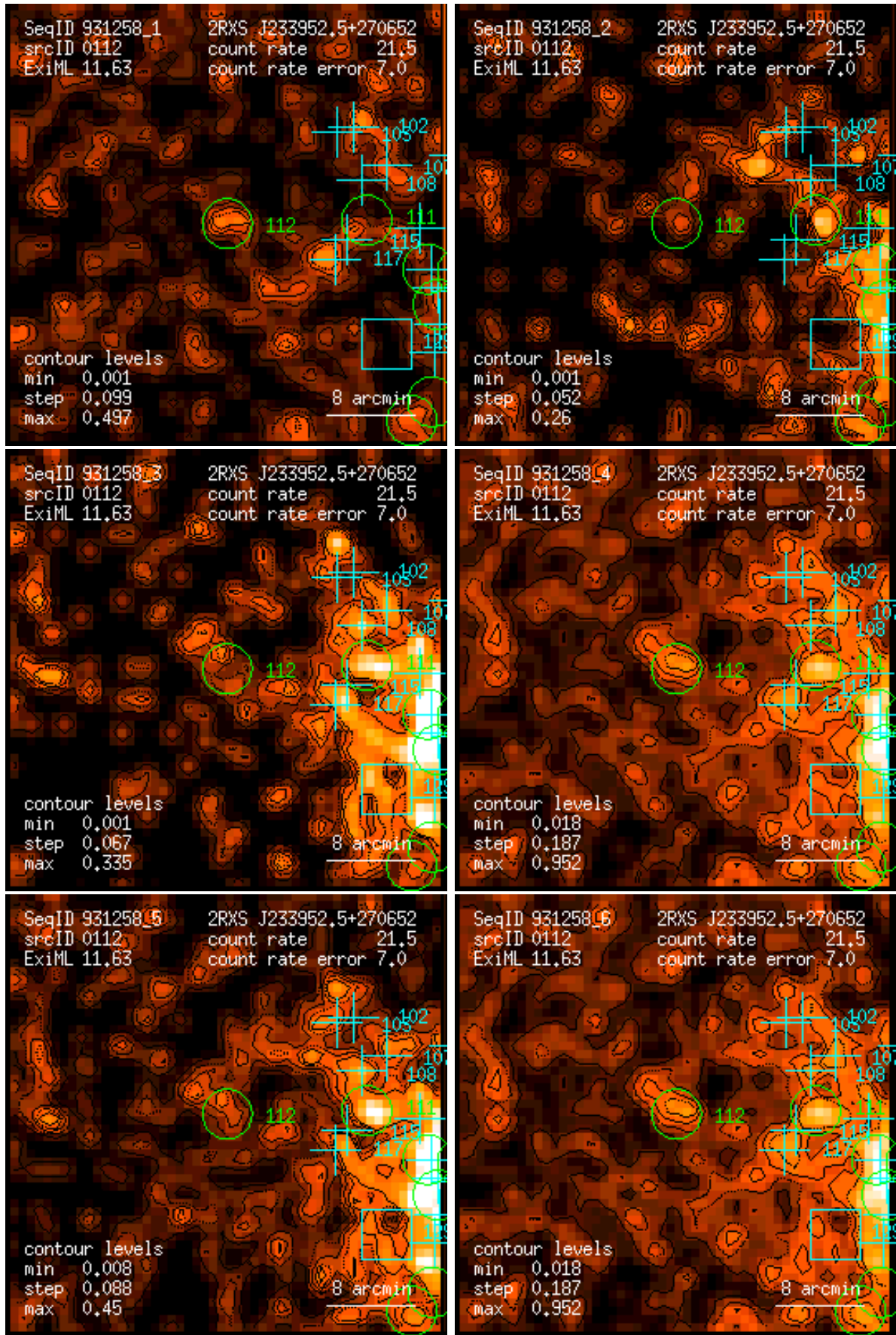
Figure 112: RASS 931258: detection 0112: band rate images, Gaussian filter: (1) PSPC channels 11 – 41, (2) 52 – 90, (3) 91 – 201, (4) 11 – 235, (5) 52 – 201, (6) 11 – 201. Broad band rates in counts/ks. Band rate contour levels in counts/ks/arcmin 2 .
