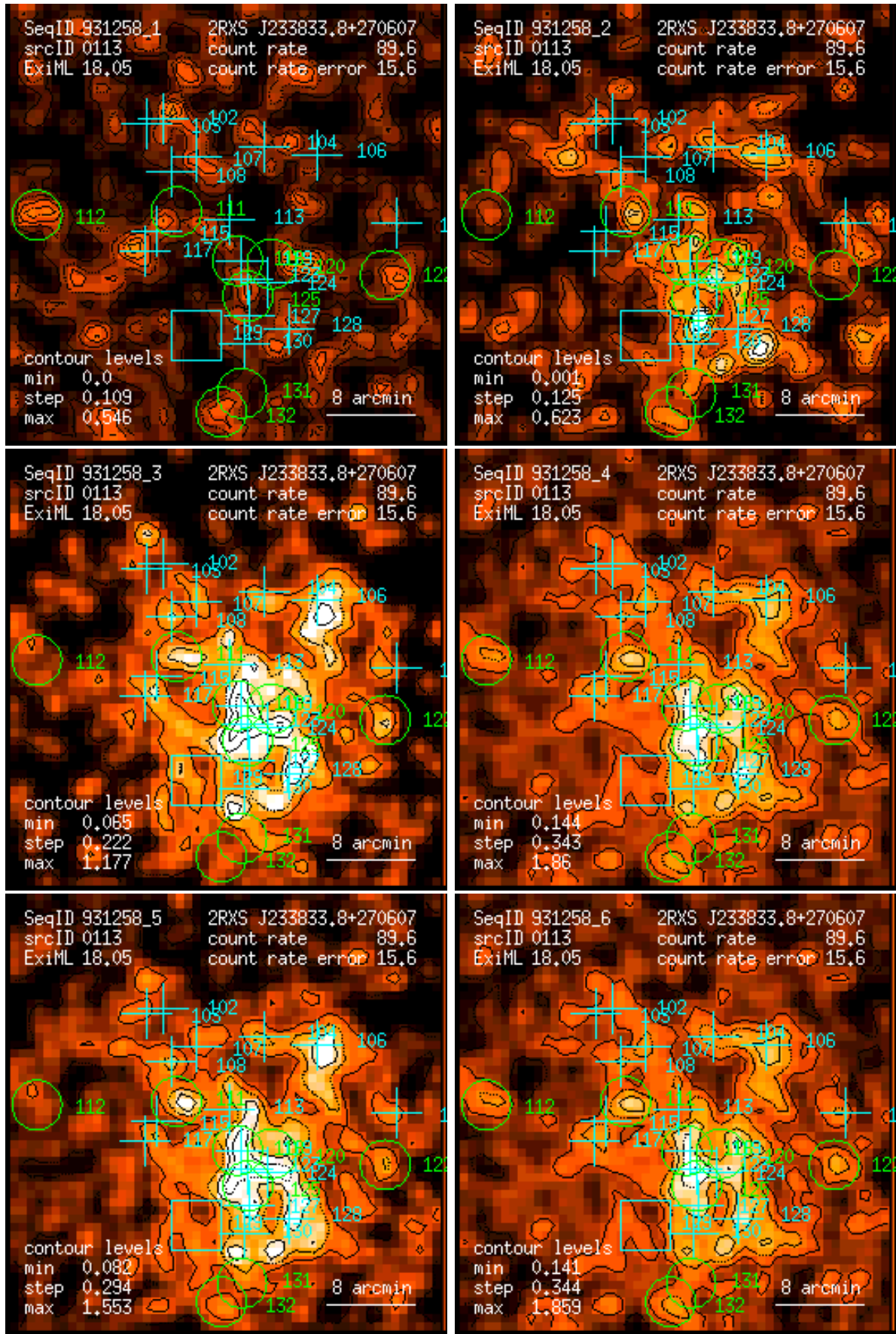
Figure 113: RASS 931258: detection 0113: band rate images, Gaussian filter: (1) PSPC channels 11 – 41, (2) 52 – 90, (3) 91 – 201, (4) 11 – 235, (5) 52 – 201, (6) 11 – 201. Broad band rates in counts/ks. Band rate contour levels in counts/ks/arcmin 2 .
