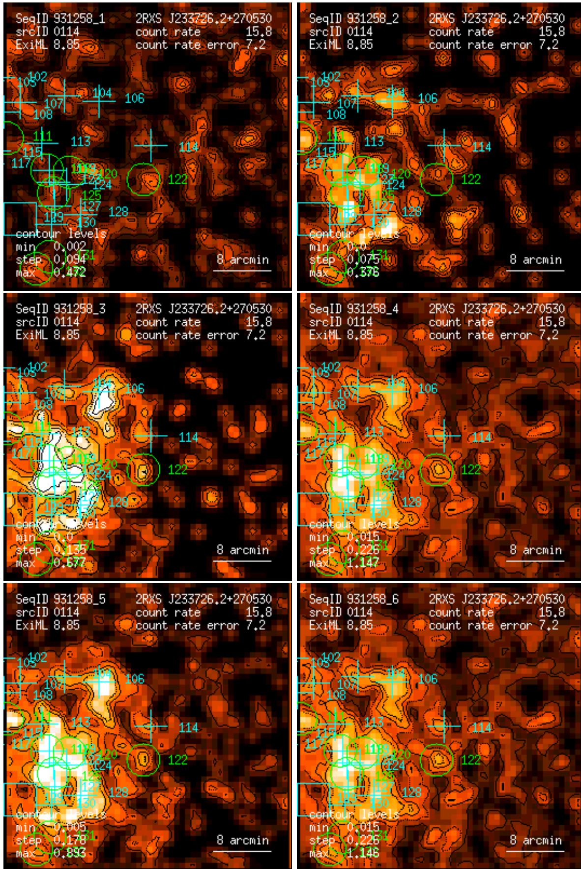
Figure 114: RASS 931258: detection 0114: band rate images, Gaussian filter: (1) PSPC channels 11 – 41, (2) 52 – 90, (3) 91 – 201, (4) 11 – 235, (5) 52 – 201, (6) 11 – 201. Broad band rates in counts/ks. Band rate contour levels in counts/ks/arcmin 2 .
