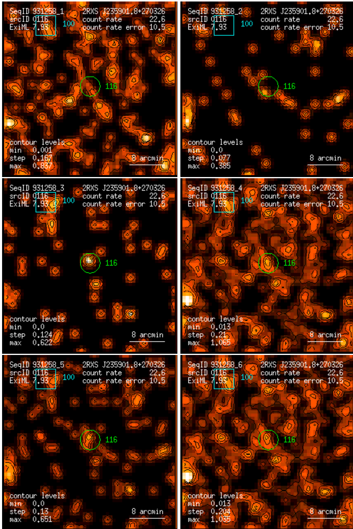
Figure 116: RASS 931258: detection 0116: band rate images, Gaussian filter: (1) PSPC channels 11 – 41, (2) 52 – 90, (3) 91 – 201, (4) 11 – 235, (5) 52 – 201, (6) 11 – 201. Broad band rates in counts/ks. Band rate contour levels in counts/ks/arcmin 2 .
