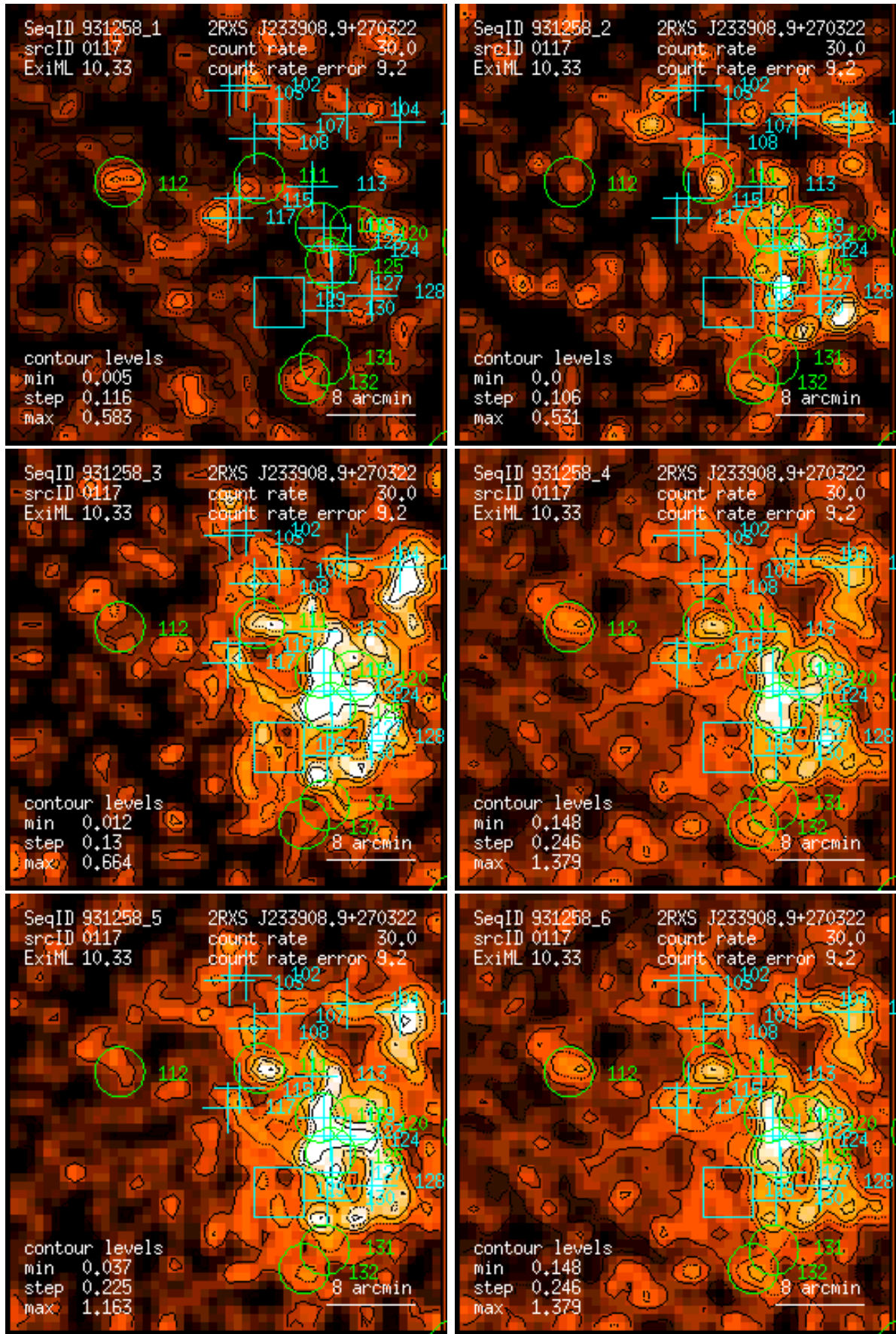
Figure 117: RASS 931258: detection 0117: band rate images, Gaussian filter: (1) PSPC channels 11 – 41, (2) 52 – 90, (3) 91 – 201, (4) 11 – 235, (5) 52 – 201, (6) 11 – 201. Broad band rates in counts/ks. Band rate contour levels in counts/ks/arcmin 2 .
