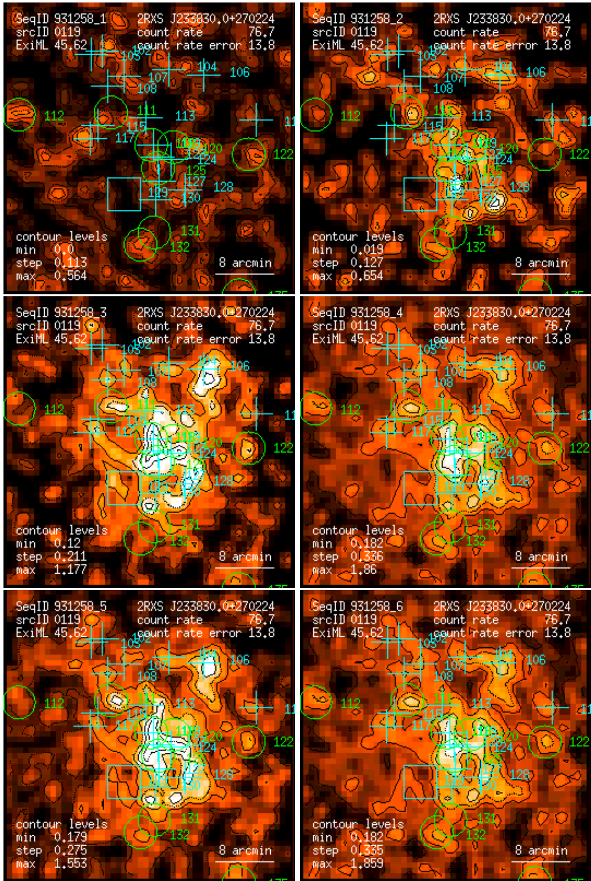
Figure 119: RASS 931258: detection 0119: band rate images, Gaussian filter: (1) PSPC channels 11 – 41, (2) 52 – 90, (3) 91 – 201, (4) 11 – 235, (5) 52 – 201, (6) 11 – 201. Broad band rates in counts/ks. Band rate contour levels in counts/ks/arcmin 2 .
