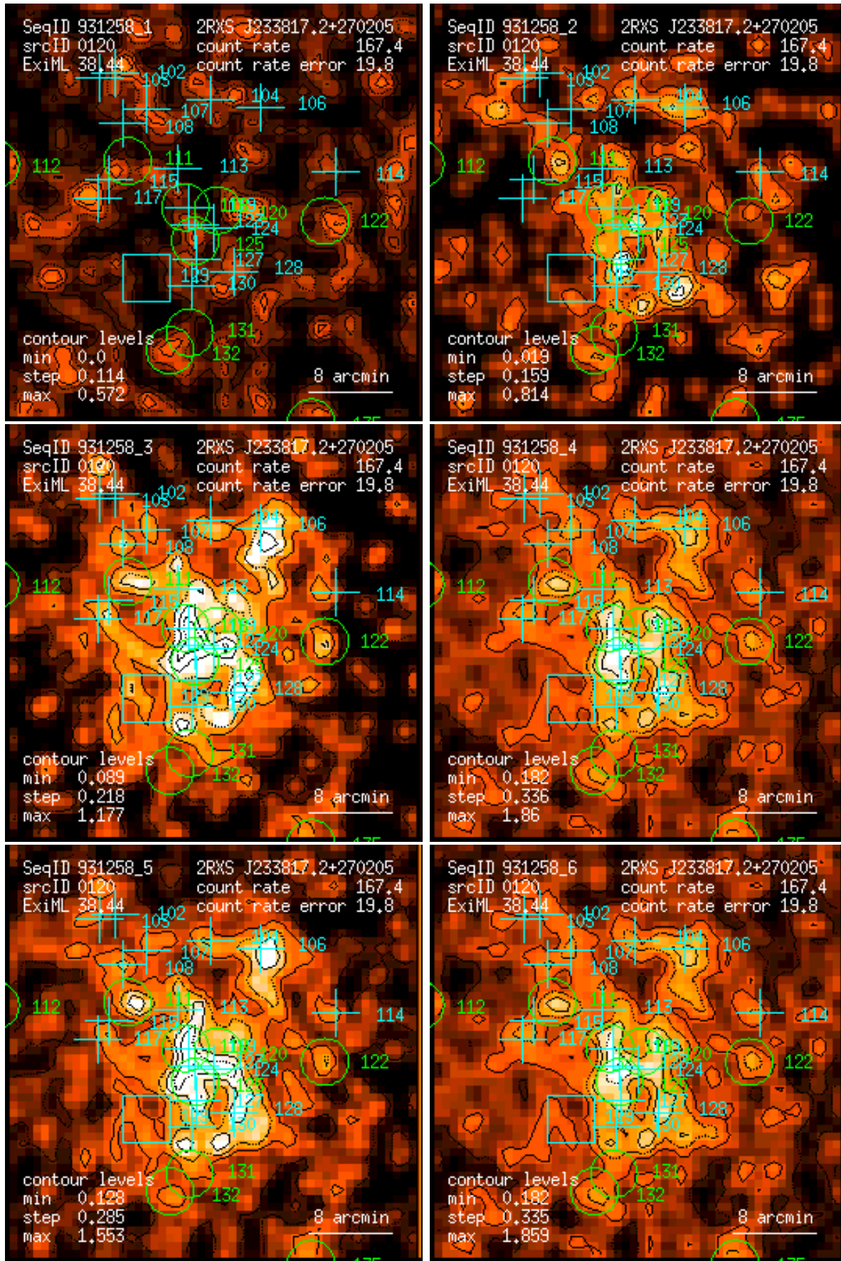
Figure 120: RASS 931258: detection 0120: band rate images, Gaussian filter: (1) PSPC channels 11 – 41, (2) 52 – 90, (3) 91 – 201, (4) 11 – 235, (5) 52 – 201, (6) 11 – 201. Broad band rates in counts/ks. Band rate contour levels in counts/ks/arcmin 2 .
