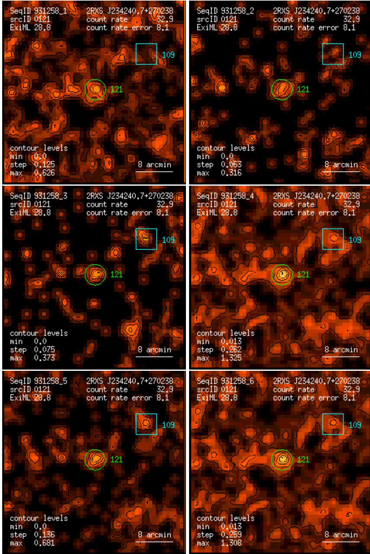
Figure 121: RASS 931258: detection 0121: band rate images, Gaussian filter: (1) PSPC channels 11 – 41, (2) 52 – 90, (3) 91 – 201, (4) 11 – 235, (5) 52 – 201, (6) 11 – 201. Broad band rates in counts/ks. Band rate contour levels in counts/ks/arcmin 2 .
