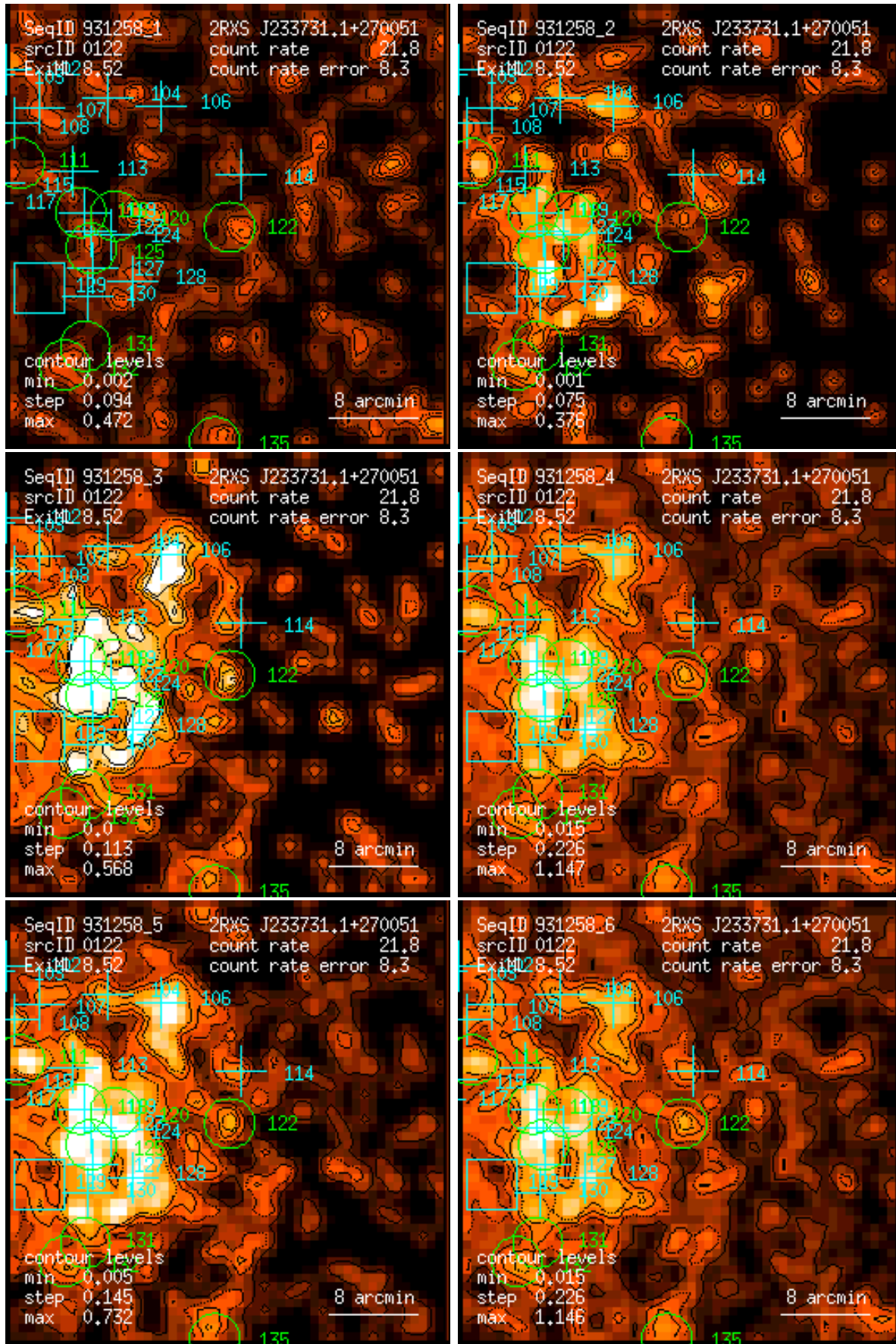
Figure 122: RASS 931258: detection 0122: band rate images, Gaussian filter: (1) PSPC channels 11 – 41, (2) 52 – 90, (3) 91 – 201, (4) 11 – 235, (5) 52 – 201, (6) 11 – 201. Broad band rates in counts/ks. Band rate contour levels in counts/ks/arcmin 2 .
