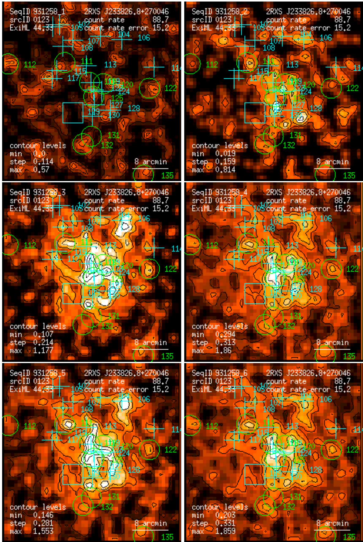
Figure 123: RASS 931258: detection 0123: band rate images, Gaussian filter: (1) PSPC channels 11 – 41, (2) 52 – 90, (3) 91 – 201, (4) 11 – 235, (5) 52 – 201, (6) 11 – 201. Broad band rates in counts/ks. Band rate contour levels in counts/ks/arcmin 2 .
