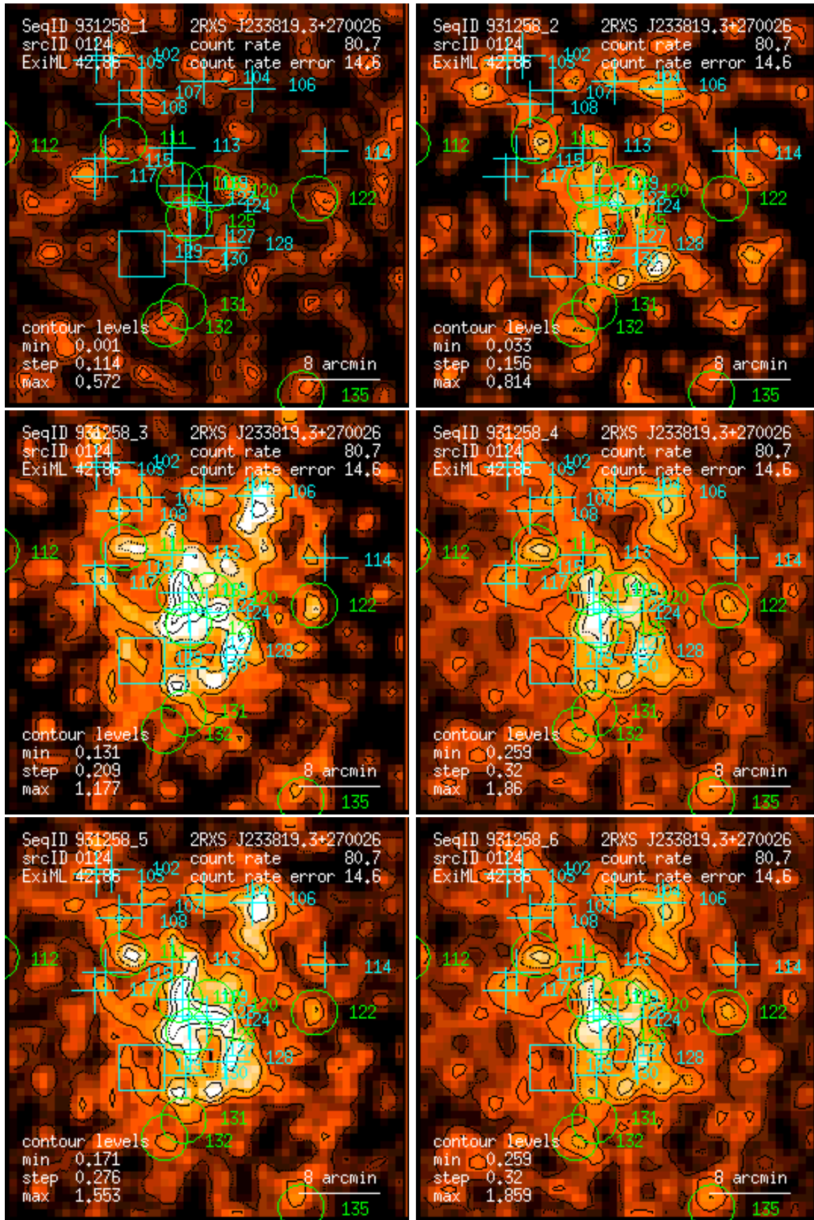
Figure 124: RASS 931258: detection 0124: band rate images, Gaussian filter: (1) PSPC channels 11 – 41, (2) 52 – 90, (3) 91 – 201, (4) 11 – 235, (5) 52 – 201, (6) 11 – 201. Broad band rates in counts/ks. Band rate contour levels in counts/ks/arcmin 2 .
