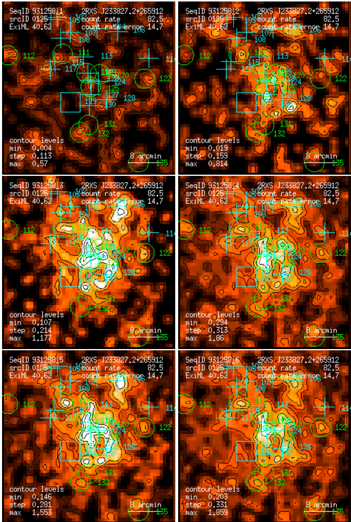
Figure 125: RASS 931258: detection 0125: band rate images, Gaussian filter: (1) PSPC channels 11 – 41, (2) 52 – 90, (3) 91 – 201, (4) 11 – 235, (5) 52 – 201, (6) 11 – 201. Broad band rates in counts/ks. Band rate contour levels in counts/ks/arcmin 2 .
