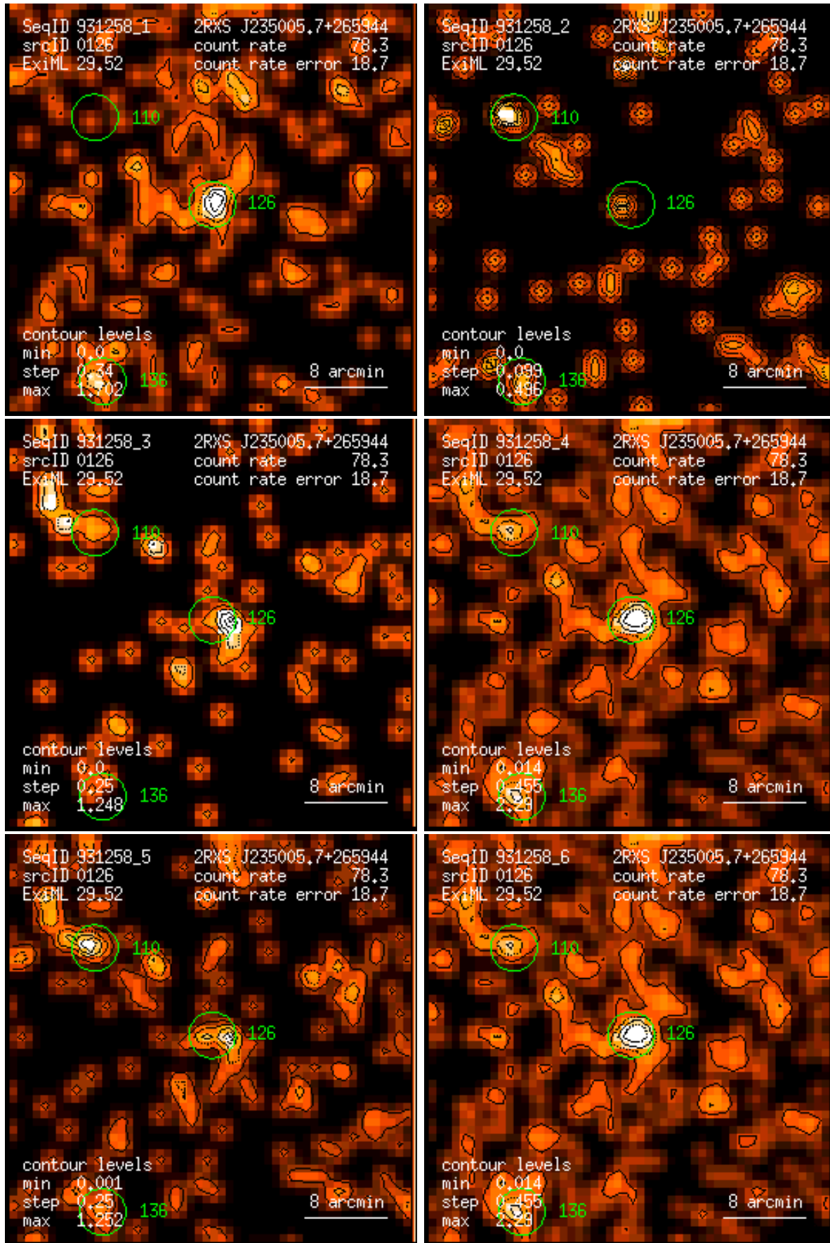
Figure 126: RASS 931258: detection 0126: band rate images, Gaussian filter: (1) PSPC channels 11 – 41, (2) 52 – 90, (3) 91 – 201, (4) 11 – 235, (5) 52 – 201, (6) 11 – 201. Broad band rates in counts/ks. Band rate contour levels in counts/ks/arcmin 2 .
