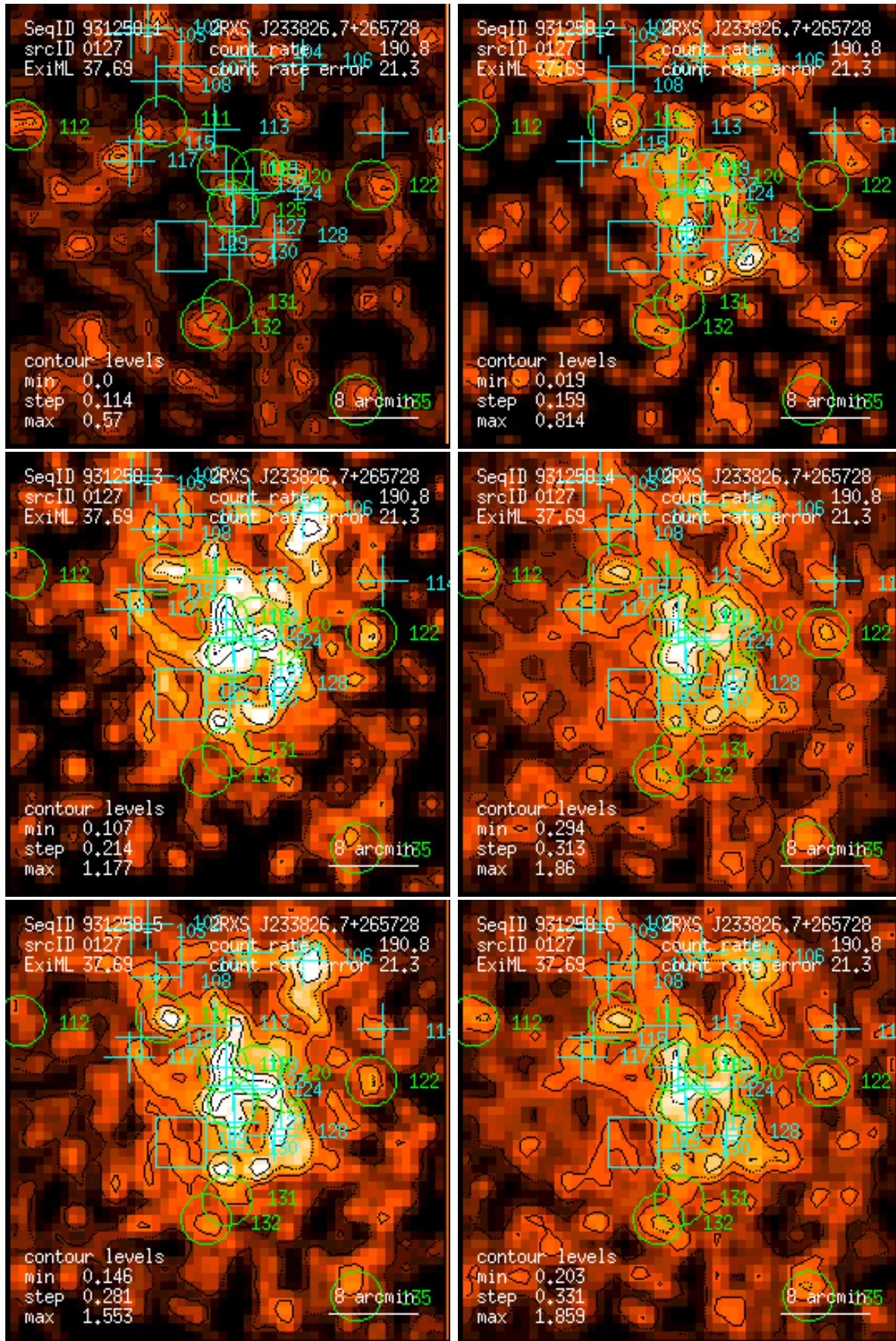
Figure 127: RASS 931258: detection 0127: band rate images, Gaussian filter: (1) PSPC channels 11 – 41, (2) 52 – 90, (3) 91 – 201, (4) 11 – 235, (5) 52 – 201, (6) 11 – 201. Broad band rates in counts/ks. Band rate contour levels in counts/ks/arcmin 2 .
