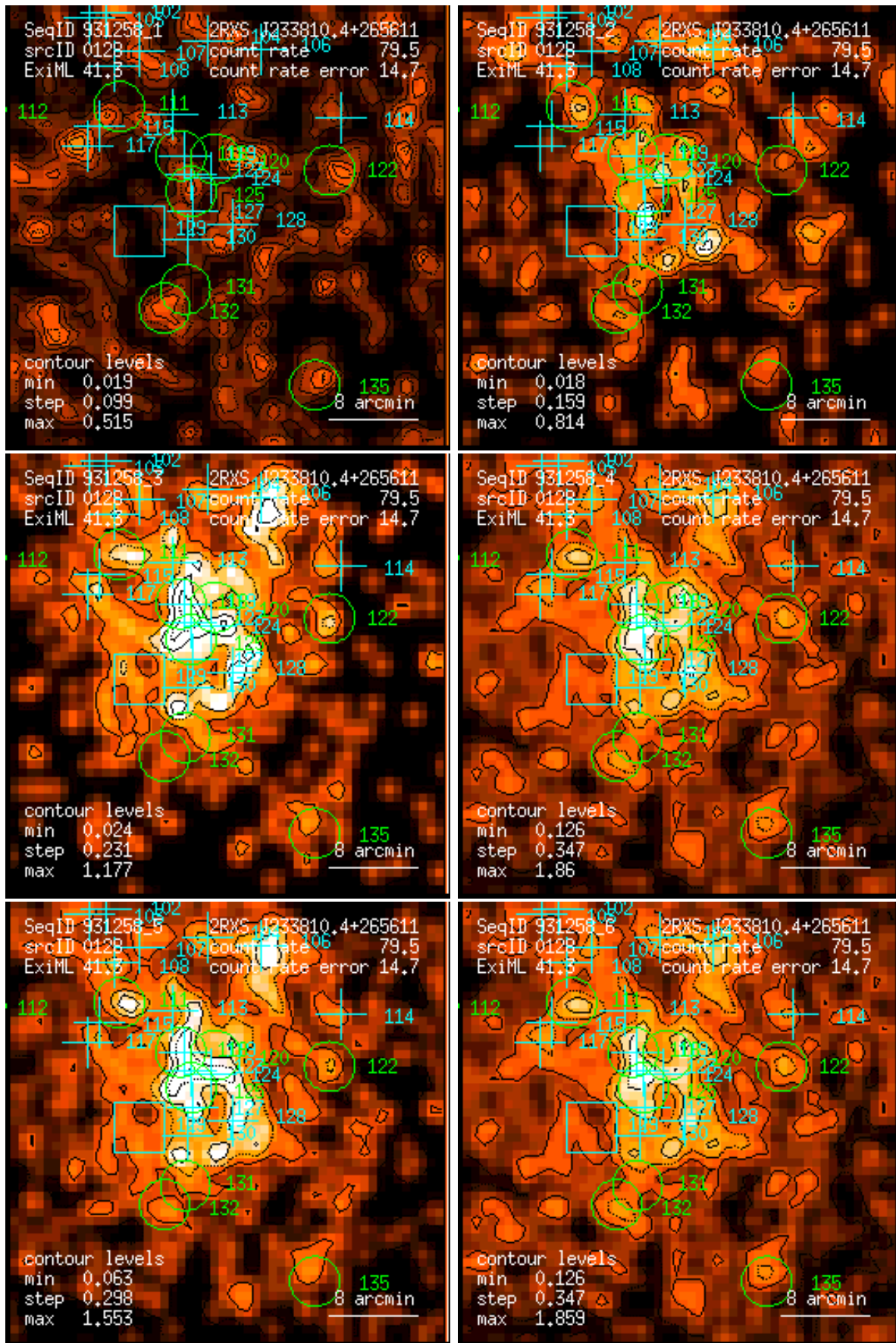
Figure 128: RASS 931258: detection 0128: band rate images, Gaussian filter: (1) PSPC channels 11 – 41, (2) 52 – 90, (3) 91 – 201, (4) 11 – 235, (5) 52 – 201, (6) 11 – 201. Broad band rates in counts/ks. Band rate contour levels in counts/ks/arcmin 2 .
