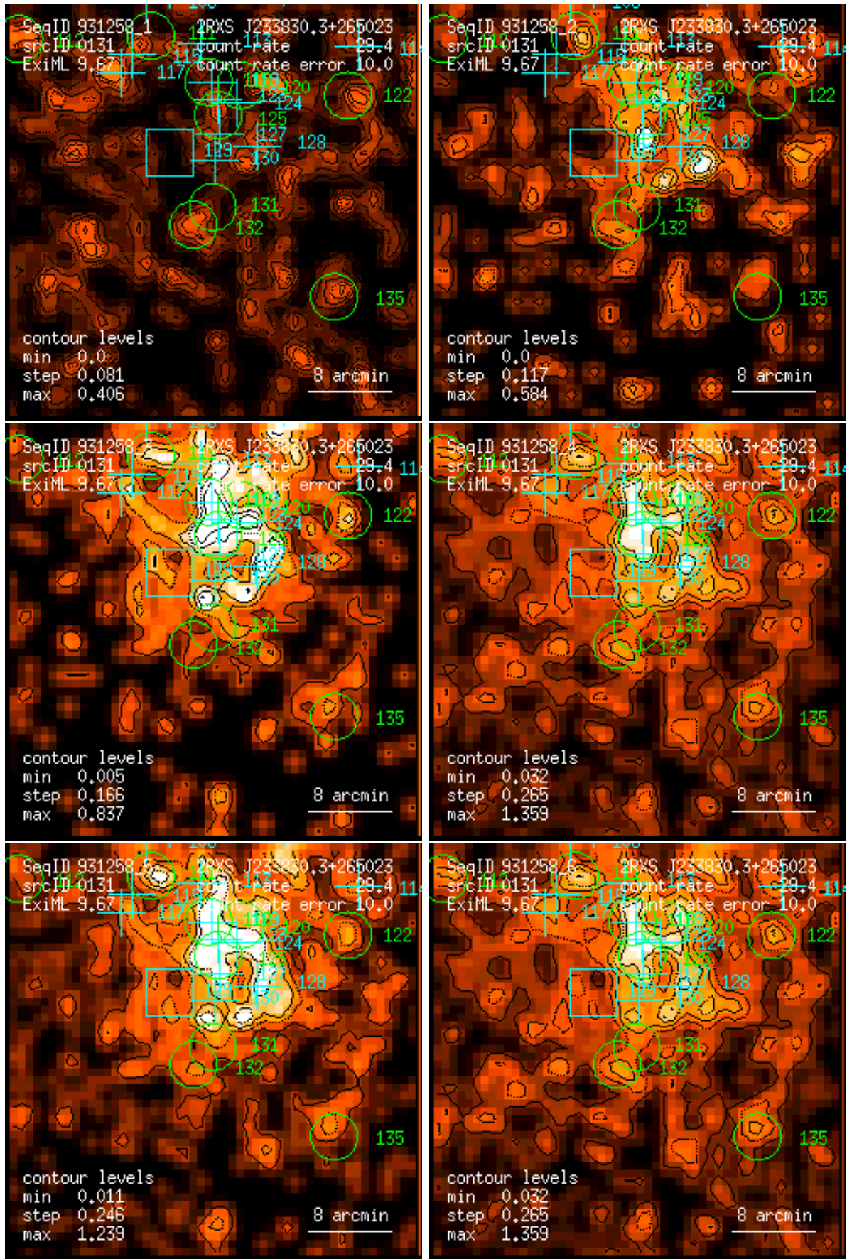
Figure 131: RASS 931258: detection 0131: band rate images, Gaussian filter: (1) PSPC channels 11 – 41, (2) 52 – 90, (3) 91 – 201, (4) 11 – 235, (5) 52 – 201, (6) 11 – 201. Broad band rates in counts/ks. Band rate contour levels in counts/ks/arcmin 2 .
