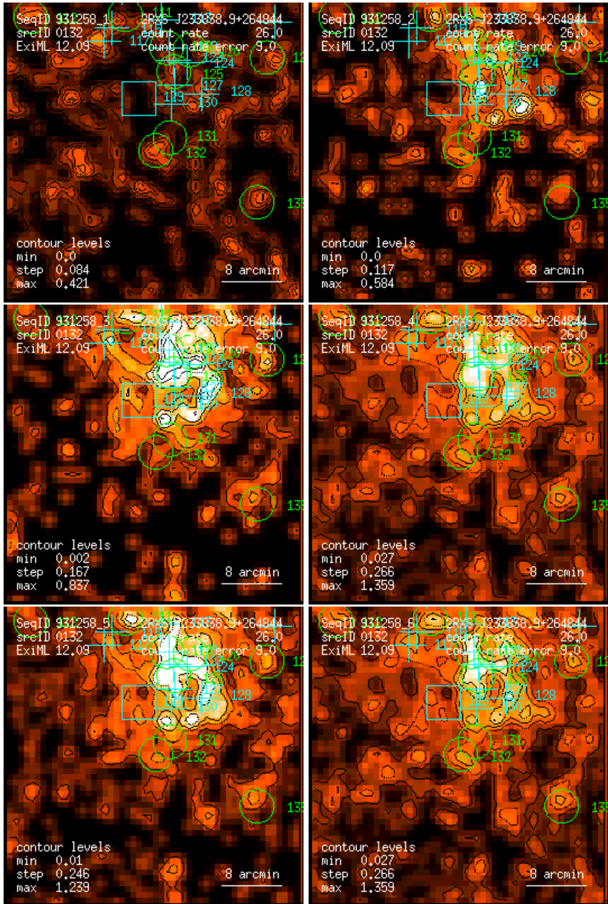
Figure 132: RASS 931258: detection 0132: band rate images, Gaussian filter: (1) PSPC channels 11 – 41, (2) 52 – 90, (3) 91 – 201, (4) 11 – 235, (5) 52 – 201, (6) 11 – 201. Broad band rates in counts/ks. Band rate contour levels in counts/ks/arcmin 2 .
